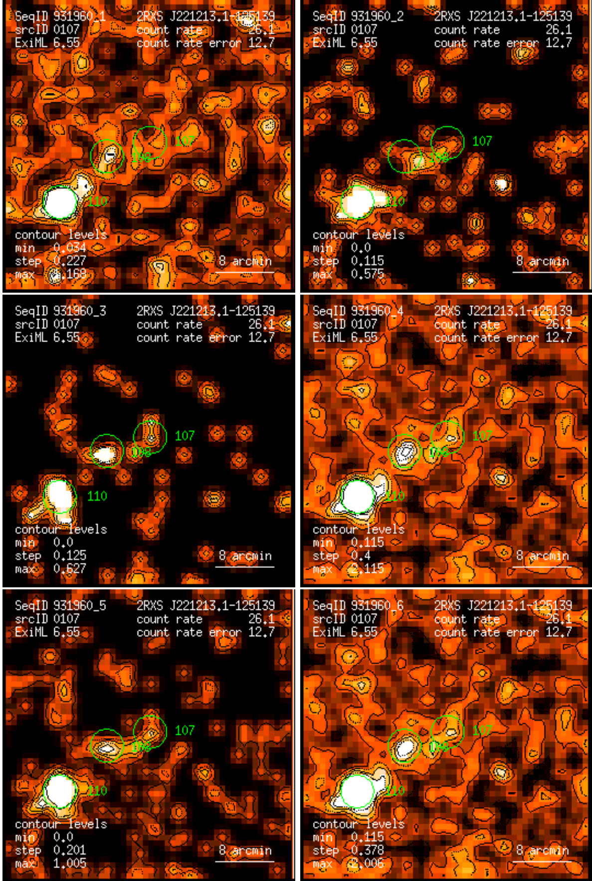
Figure 107: RASS 931960: detection 0107: band rate images, Gaussian filter: (1) PSPC channels 11 – 41, (2) 52 – 90, (3) 91 – 201, (4) 11 – 235, (5) 52 – 201, (6) 11 – 201. Broad band rates in counts/ks. Band rate contour levels in counts/ks/arcmin 2 .
