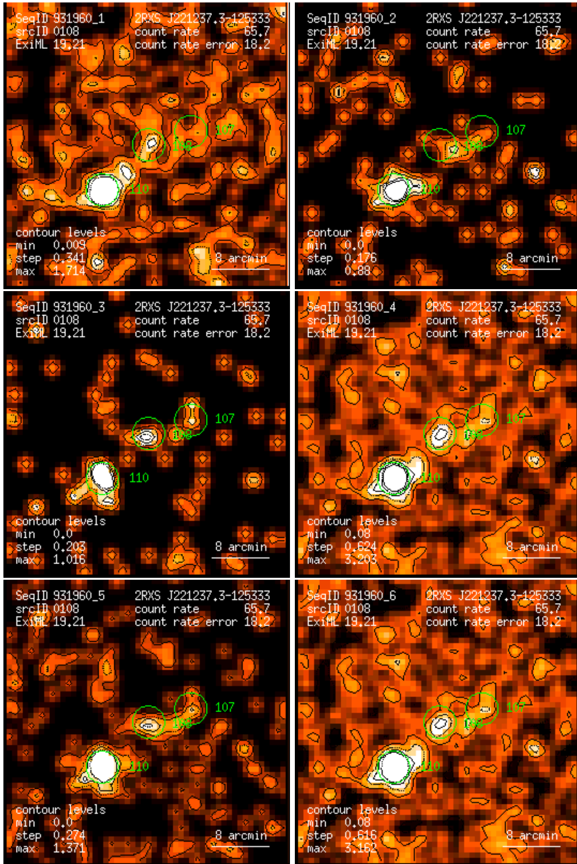
Figure 108: RASS 931960: detection 0108: band rate images, Gaussian filter: (1) PSPC channels 11 – 41, (2) 52 – 90, (3) 91 – 201, (4) 11 – 235, (5) 52 – 201, (6) 11 – 201. Broad band rates in counts/ks. Band rate contour levels in counts/ks/arcmin 2 .
