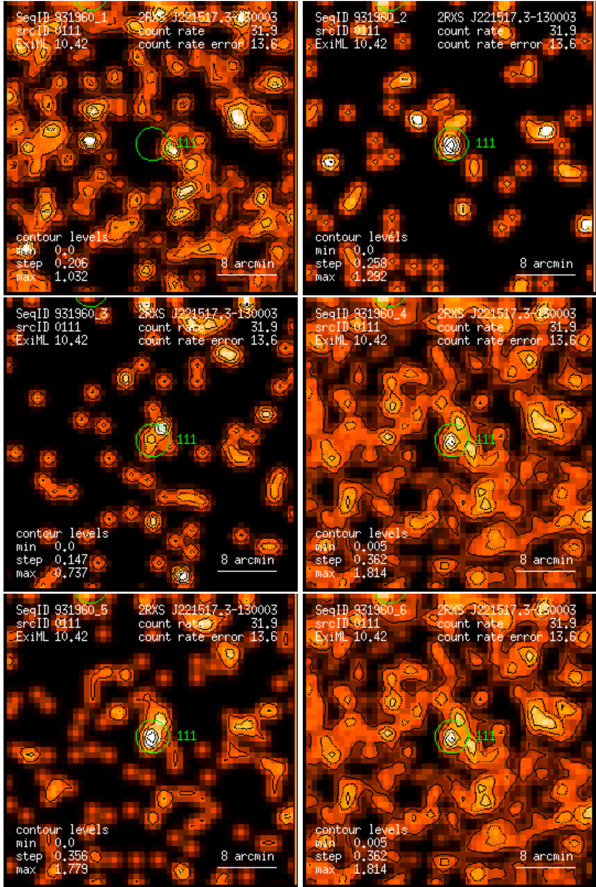
Figure 111: RASS 931960: detection 0111: band rate images, Gaussian filter: (1) PSPC channels 11 – 41, (2) 52 – 90, (3) 91 – 201, (4) 11 – 235, (5) 52 – 201, (6) 11 – 201. Broad band rates in counts/ks. Band rate contour levels in counts/ks/arcmin 2 .
