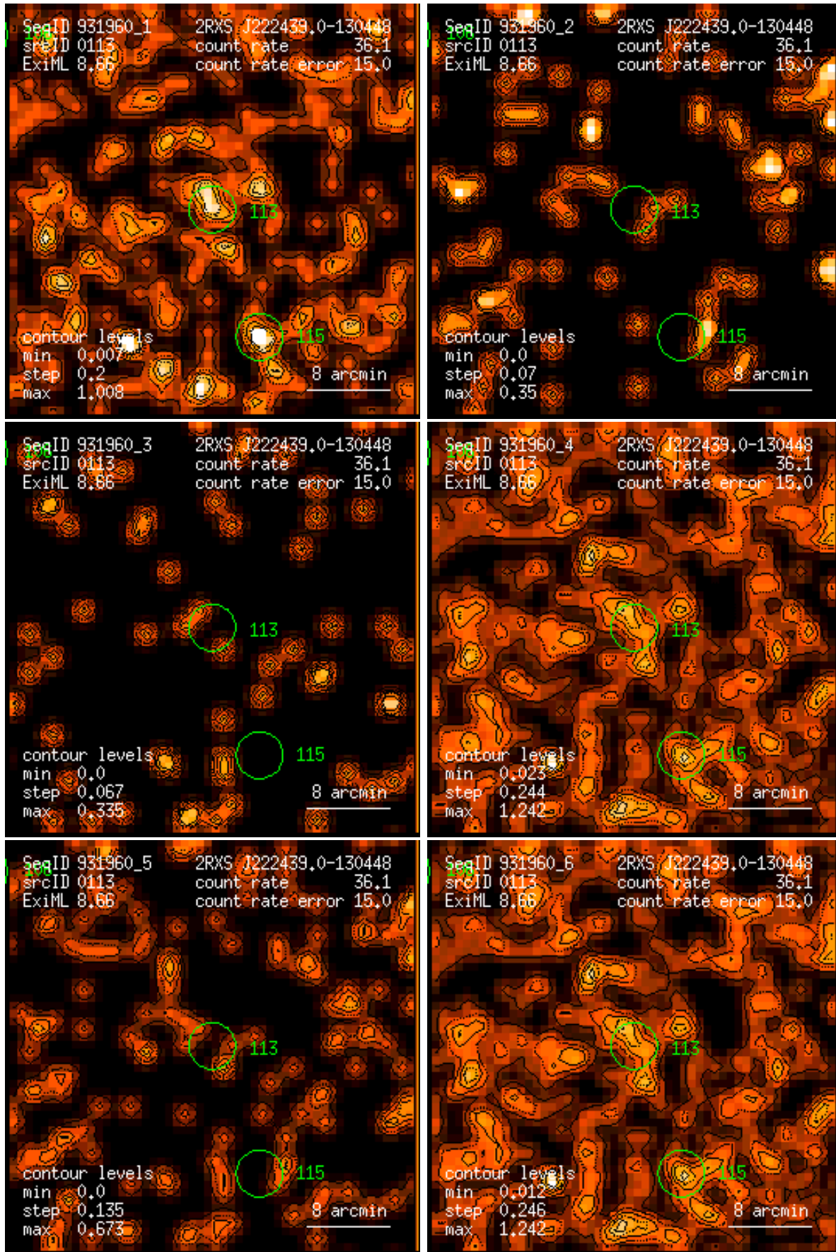
Figure 113: RASS 931960: detection 0113: band rate images, Gaussian filter: (1) PSPC channels 11 – 41, (2) 52 – 90, (3) 91 – 201, (4) 11 – 235, (5) 52 – 201, (6) 11 – 201. Broad band rates in counts/ks. Band rate contour levels in counts/ks/arcmin 2 .
