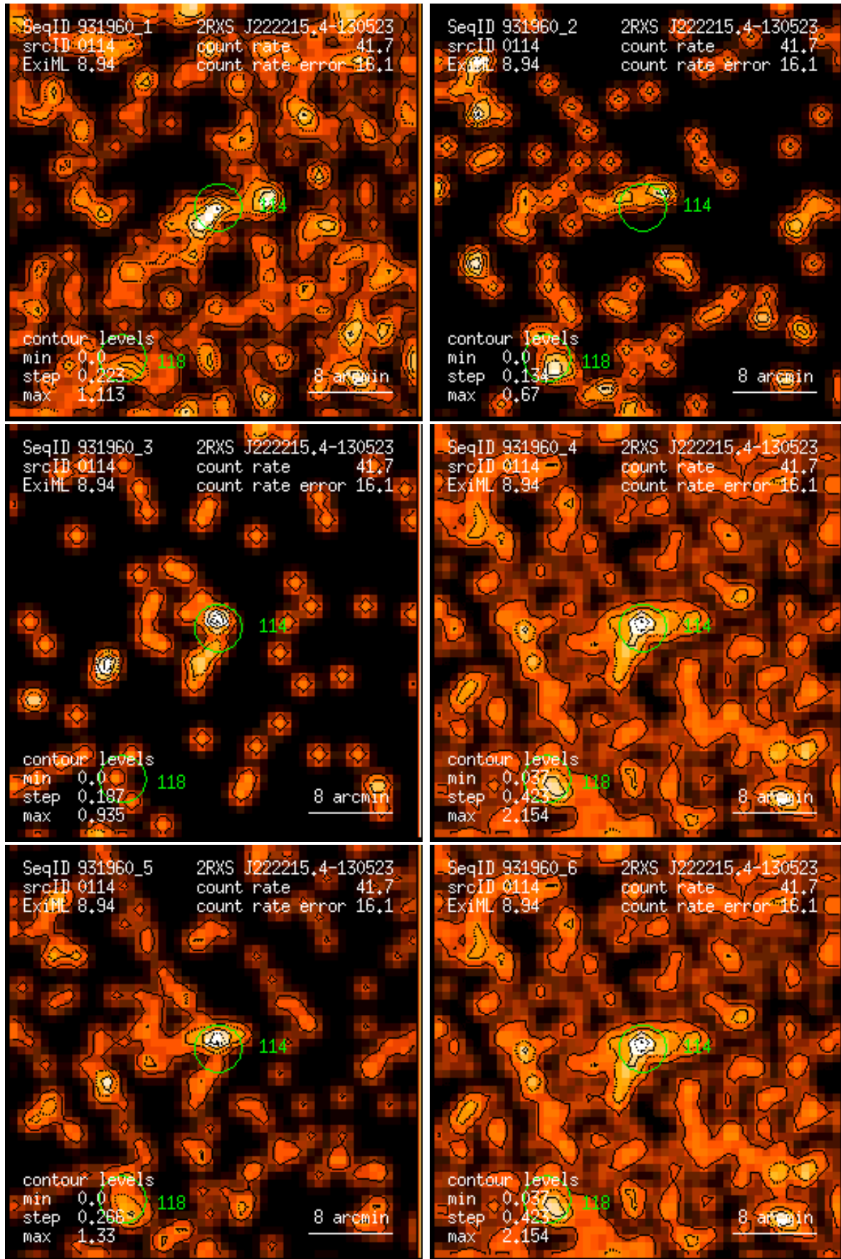
Figure 114: RASS 931960: detection 0114: band rate images, Gaussian filter: (1) PSPC channels 11 – 41, (2) 52 – 90, (3) 91 – 201, (4) 11 – 235, (5) 52 – 201, (6) 11 – 201. Broad band rates in counts/ks. Band rate contour levels in counts/ks/arcmin 2 .
