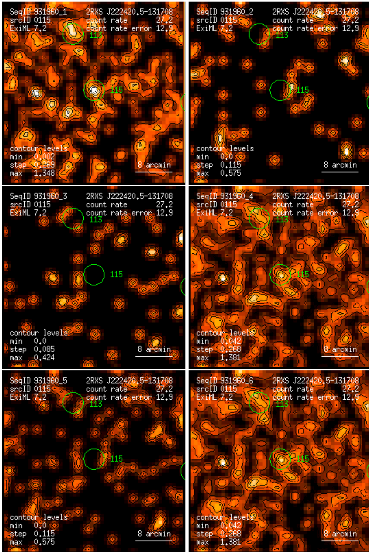
Figure 115: RASS 931960: detection 0115: band rate images, Gaussian filter: (1) PSPC channels 11 – 41, (2) 52 – 90, (3) 91 – 201, (4) 11 – 235, (5) 52 – 201, (6) 11 – 201. Broad band rates in counts/ks. Band rate contour levels in counts/ks/arcmin 2 .
