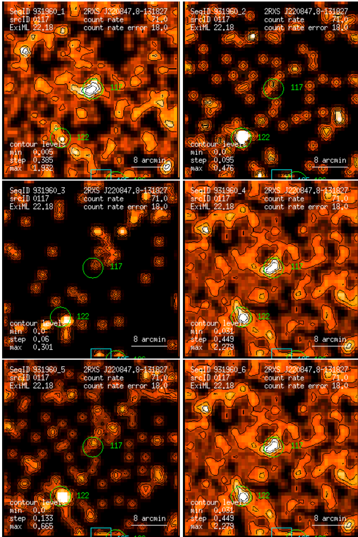
Figure 117: RASS 931960: detection 0117: band rate images, Gaussian filter: (1) PSPC channels 11 – 41, (2) 52 – 90, (3) 91 – 201, (4) 11 – 235, (5) 52 – 201, (6) 11 – 201. Broad band rates in counts/ks. Band rate contour levels in counts/ks/arcmin 2 .
