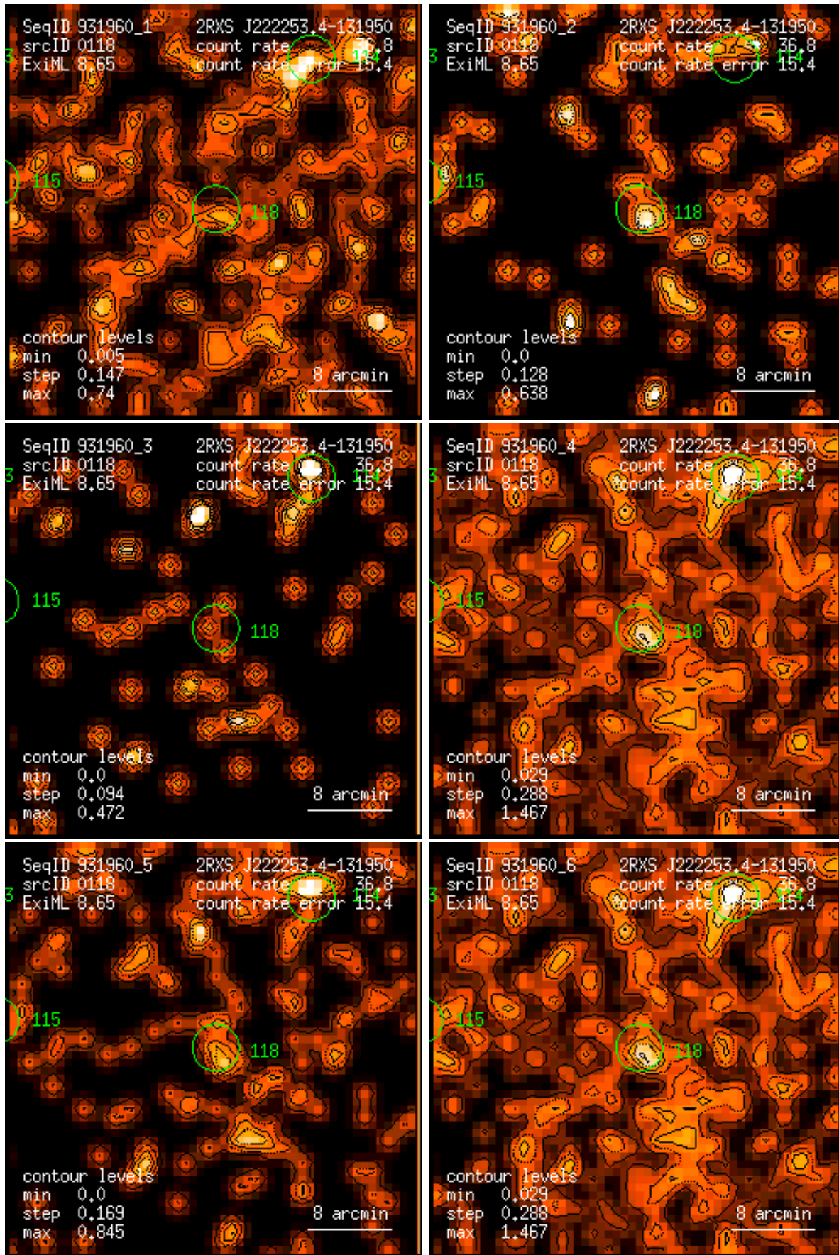
Figure 118: RASS 931960: detection 0118: band rate images, Gaussian filter: (1) PSPC channels 11 – 41, (2) 52 – 90, (3) 91 – 201, (4) 11 – 235, (5) 52 – 201, (6) 11 – 201. Broad band rates in counts/ks. Band rate contour levels in counts/ks/arcmin 2 .
