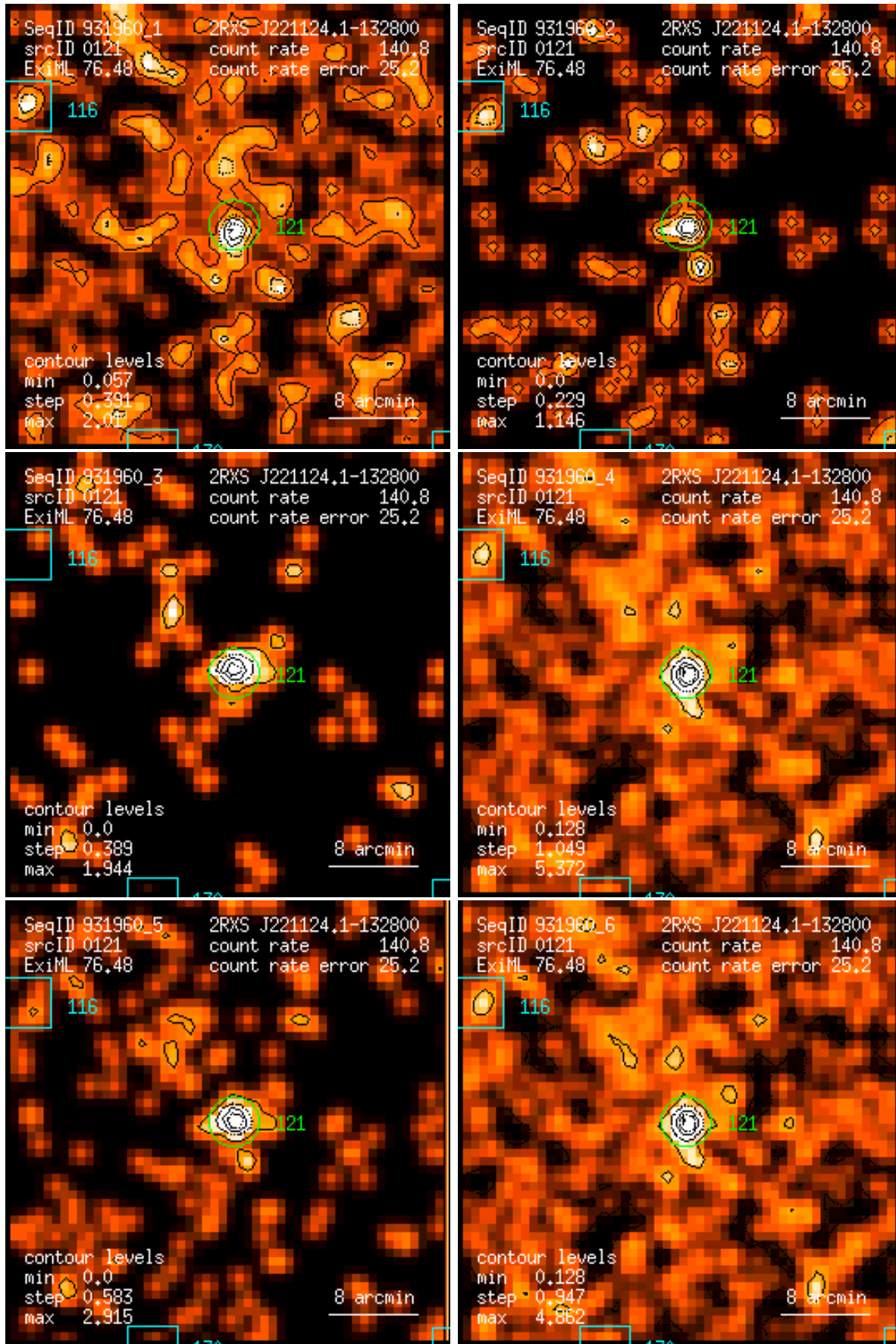
Figure 121: RASS 931960: detection 0121: band rate images, Gaussian filter: (1) PSPC channels 11 – 41, (2) 52 – 90, (3) 91 – 201, (4) 11 – 235, (5) 52 – 201, (6) 11 – 201. Broad band rates in counts/ks. Band rate contour levels in counts/ks/arcmin 2 .
