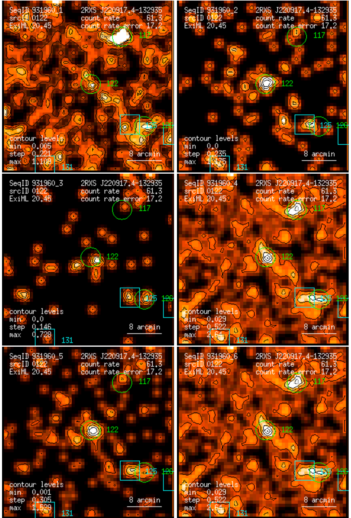
Figure 122: RASS 931960: detection 0122: band rate images, Gaussian filter: (1) PSPC channels 11 – 41, (2) 52 – 90, (3) 91 – 201, (4) 11 – 235, (5) 52 – 201, (6) 11 – 201. Broad band rates in counts/ks. Band rate contour levels in counts/ks/arcmin 2 .
