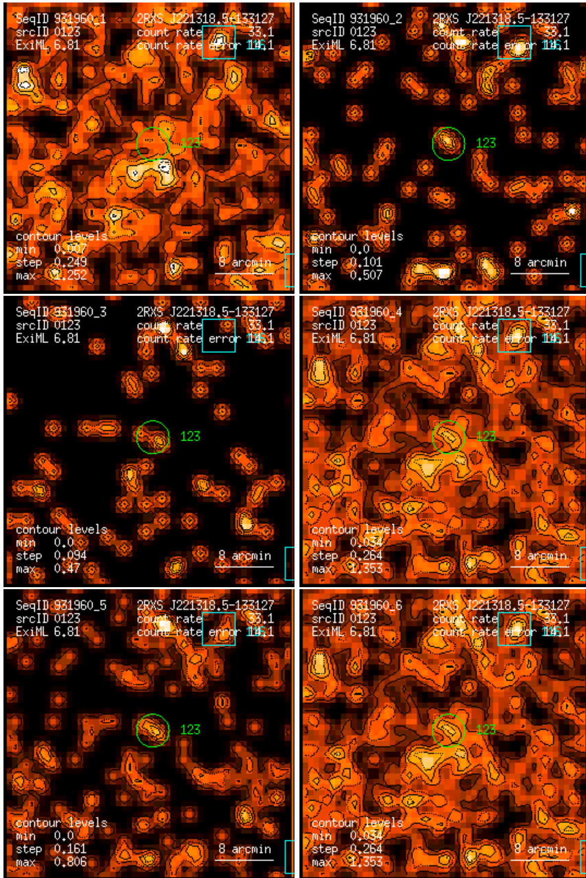
Figure 123: RASS 931960: detection 0123: band rate images, Gaussian filter: (1) PSPC channels 11 – 41, (2) 52 – 90, (3) 91 – 201, (4) 11 – 235, (5) 52 – 201, (6) 11 – 201. Broad band rates in counts/ks. Band rate contour levels in counts/ks/arcmin 2 .
