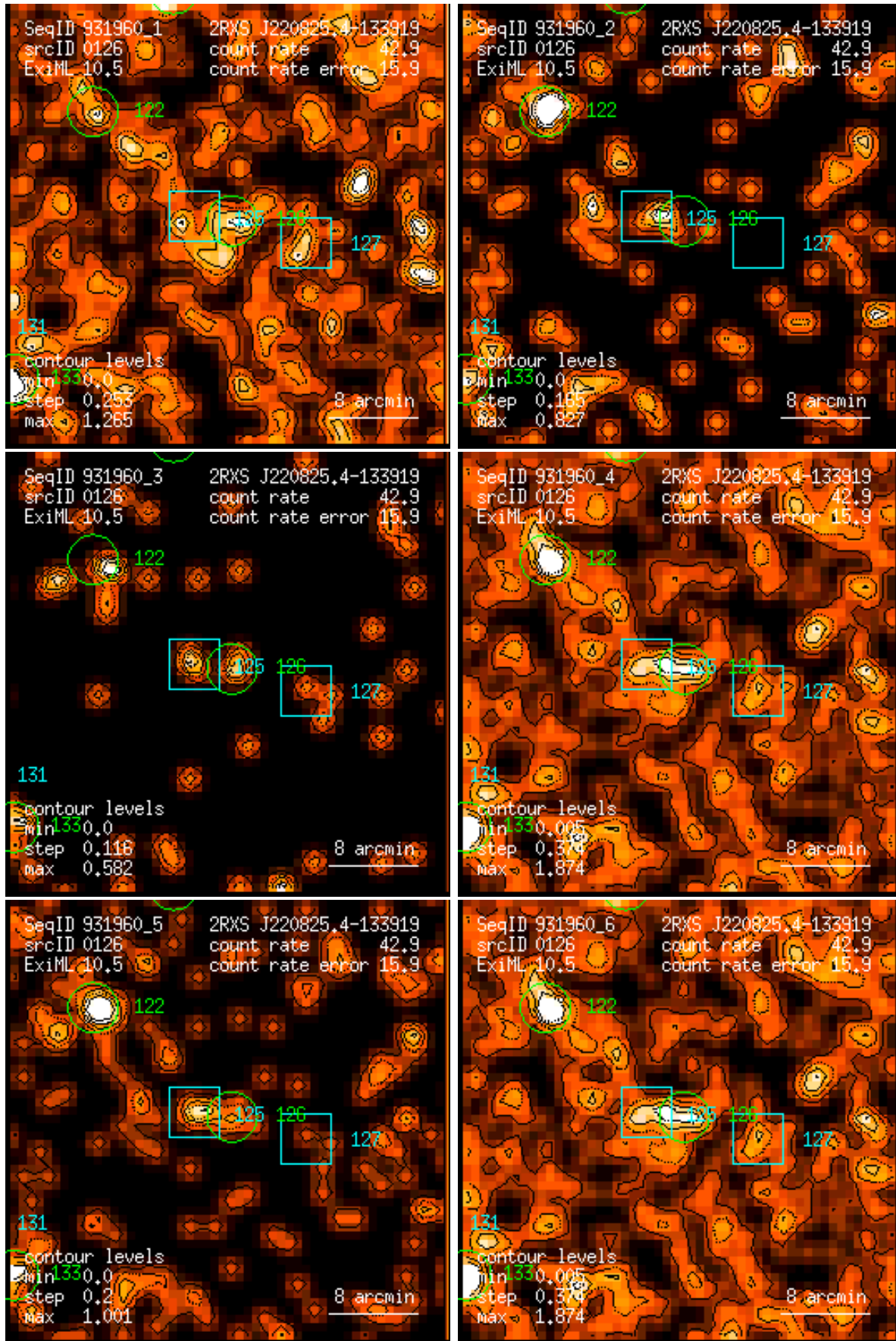
Figure 126: RASS 931960: detection 0126: band rate images, Gaussian filter: (1) PSPC channels 11 – 41, (2) 52 – 90, (3) 91 – 201, (4) 11 – 235, (5) 52 – 201, (6) 11 – 201. Broad band rates in counts/ks. Band rate contour levels in counts/ks/arcmin 2 .
