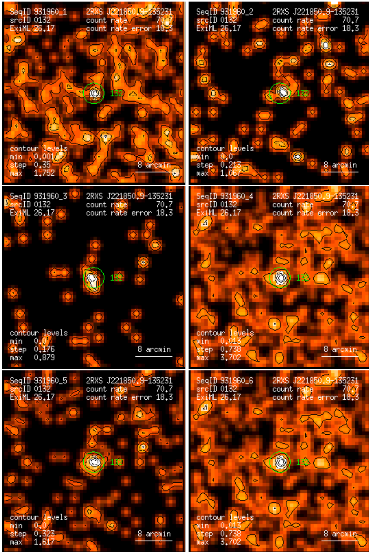
Figure 132: RASS 931960: detection 0132: band rate images, Gaussian filter: (1) PSPC channels 11 – 41, (2) 52 – 90, (3) 91 – 201, (4) 11 – 235, (5) 52 – 201, (6) 11 – 201. Broad band rates in counts/ks. Band rate contour levels in counts/ks/arcmin 2 .
