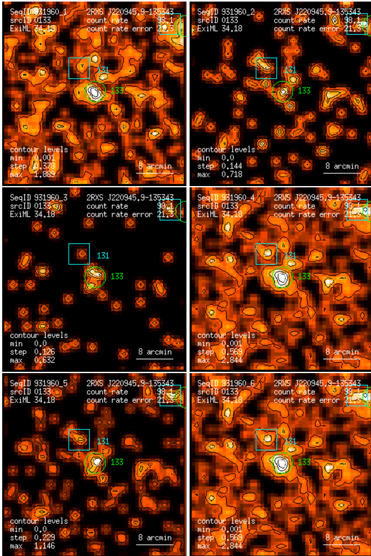
Figure 133: RASS 931960: detection 0133: band rate images, Gaussian filter: (1) PSPC channels 11 – 41, (2) 52 – 90, (3) 91 – 201, (4) 11 – 235, (5) 52 – 201, (6) 11 – 201. Broad band rates in counts/ks. Band rate contour levels in counts/ks/arcmin 2 .
