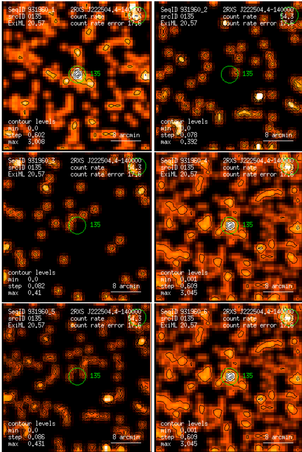
Figure 135: RASS 931960: detection 0135: band rate images, Gaussian filter: (1) PSPC channels 11 – 41, (2) 52 – 90, (3) 91 – 201, (4) 11 – 235, (5) 52 – 201, (6) 11 – 201. Broad band rates in counts/ks. Band rate contour levels in counts/ks/arcmin 2 .
