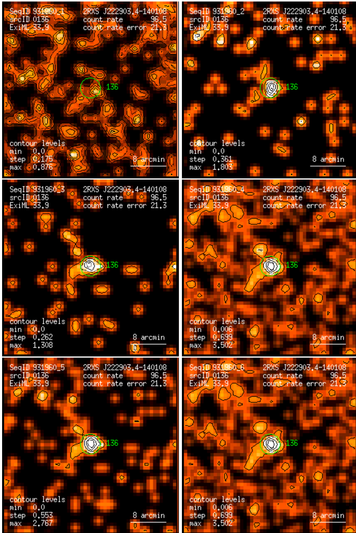
Figure 136: RASS 931960: detection 0136: band rate images, Gaussian filter: (1) PSPC channels 11 – 41, (2) 52 – 90, (3) 91 – 201, (4) 11 – 235, (5) 52 – 201, (6) 11 – 201. Broad band rates in counts/ks. Band rate contour levels in counts/ks/arcmin 2 .
