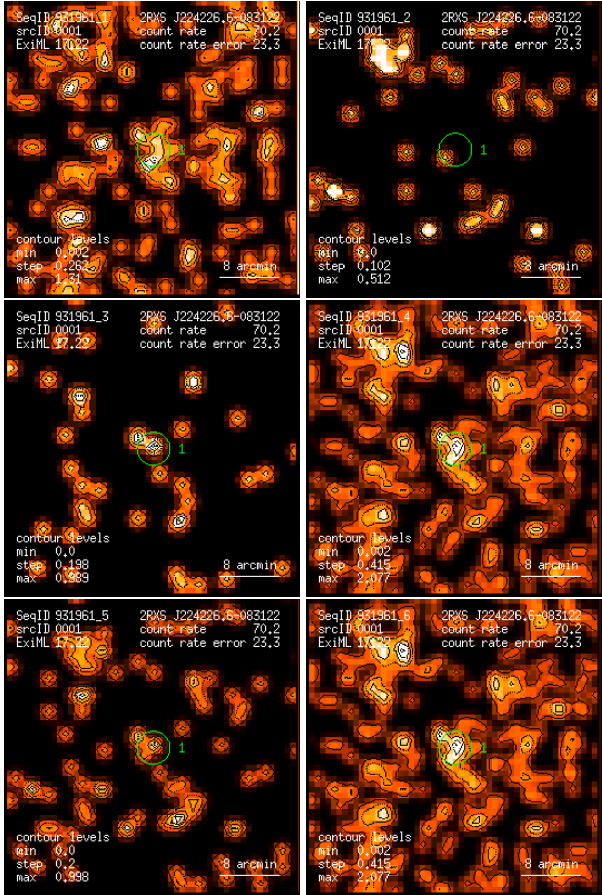
Figure 1: RASS 931961: detection 0001: band rate images, Gaussian filter: (1) PSPC channels 11 – 41, (2) 52 – 90, (3) 91 – 201, (4) 11 – 235, (5) 52 – 201, (6) 11 – 201. Broad band rates in counts/ks. Band rate contour levels in counts/ks/arcmin 2 .
