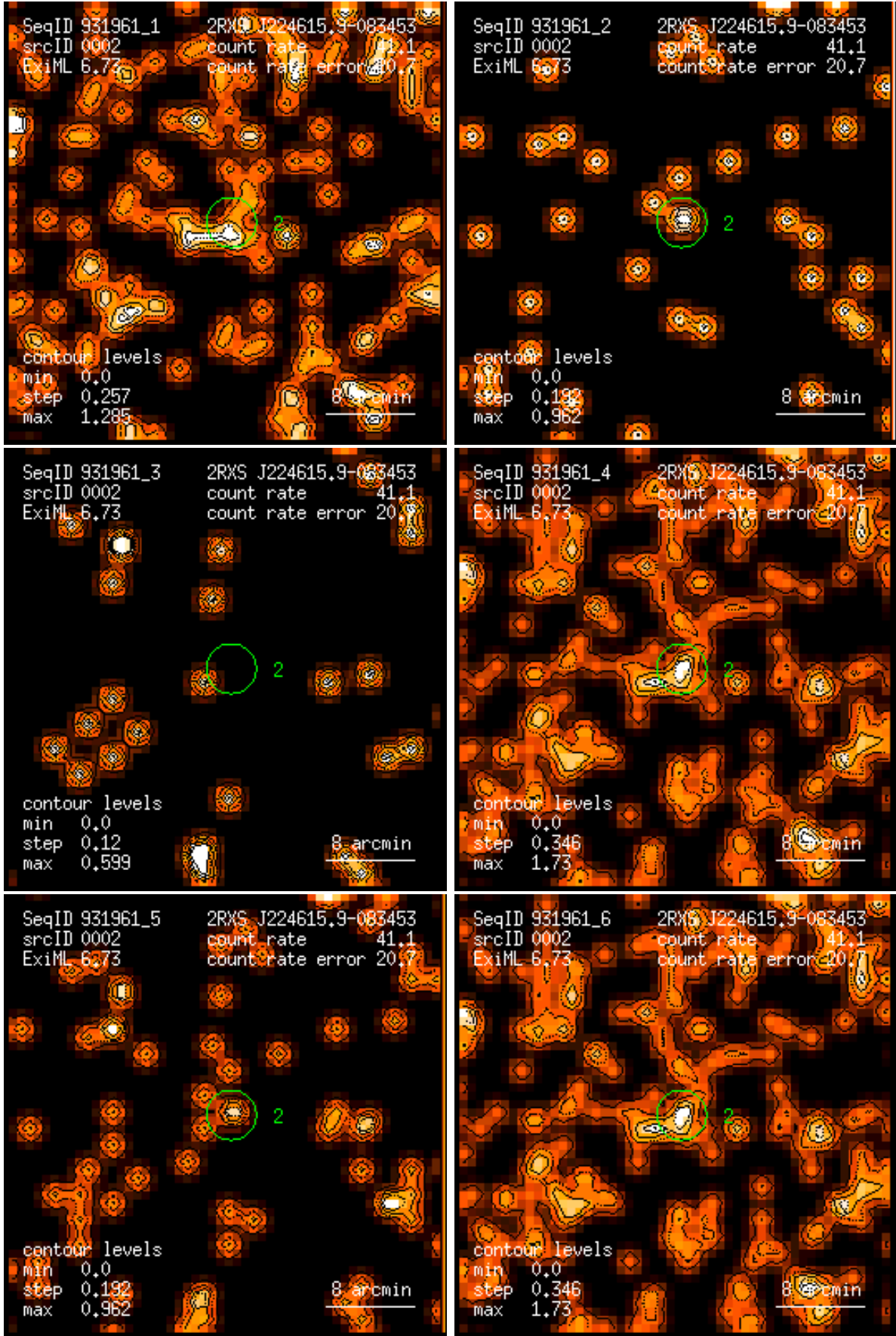
Figure 2: RASS 931961: detection 0002: band rate images, Gaussian filter: (1) PSPC channels 11 – 41, (2) 52 – 90, (3) 91 – 201, (4) 11 – 235, (5) 52 – 201, (6) 11 – 201. Broad band rates in counts/ks. Band rate contour levels in counts/ks/arcmin 2 .
