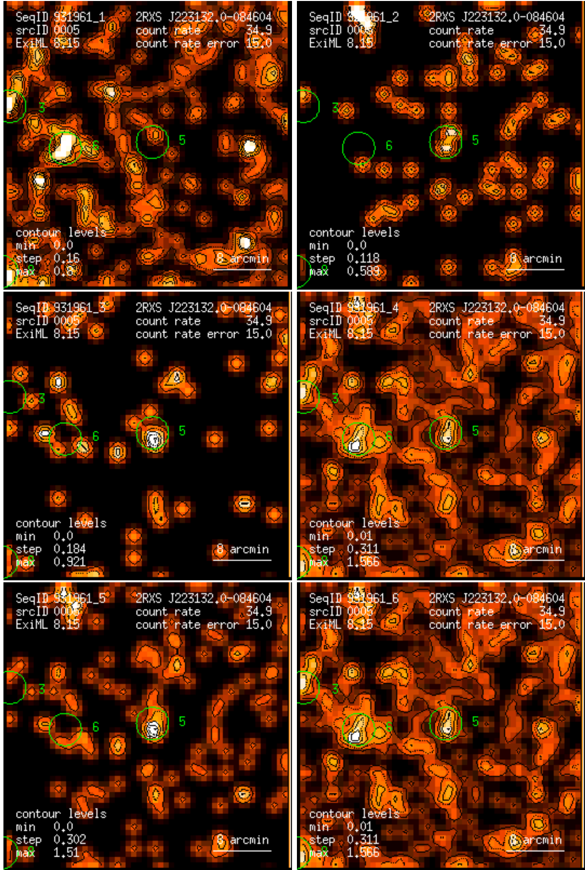
Figure 5: RASS 931961: detection 0005: band rate images, Gaussian filter: (1) PSPC channels 11 – 41, (2) 52 – 90, (3) 91 – 201, (4) 11 – 235, (5) 52 – 201, (6) 11 – 201. Broad band rates in counts/ks. Band rate contour levels in counts/ks/arcmin 2 .
