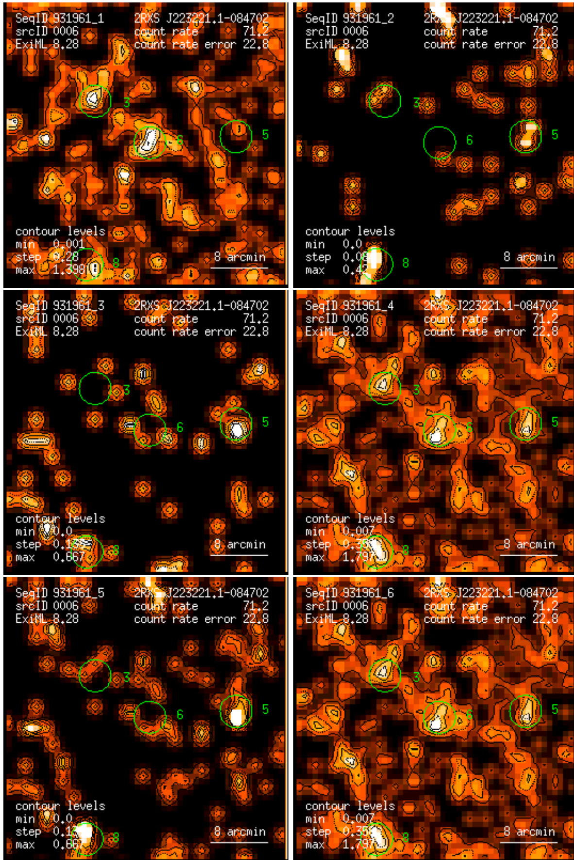
Figure 6: RASS 931961: detection 0006: band rate images, Gaussian filter: (1) PSPC channels 11 – 41, (2) 52 – 90, (3) 91 – 201, (4) 11 – 235, (5) 52 – 201, (6) 11 – 201. Broad band rates in counts/ks. Band rate contour levels in counts/ks/arcmin 2 .
