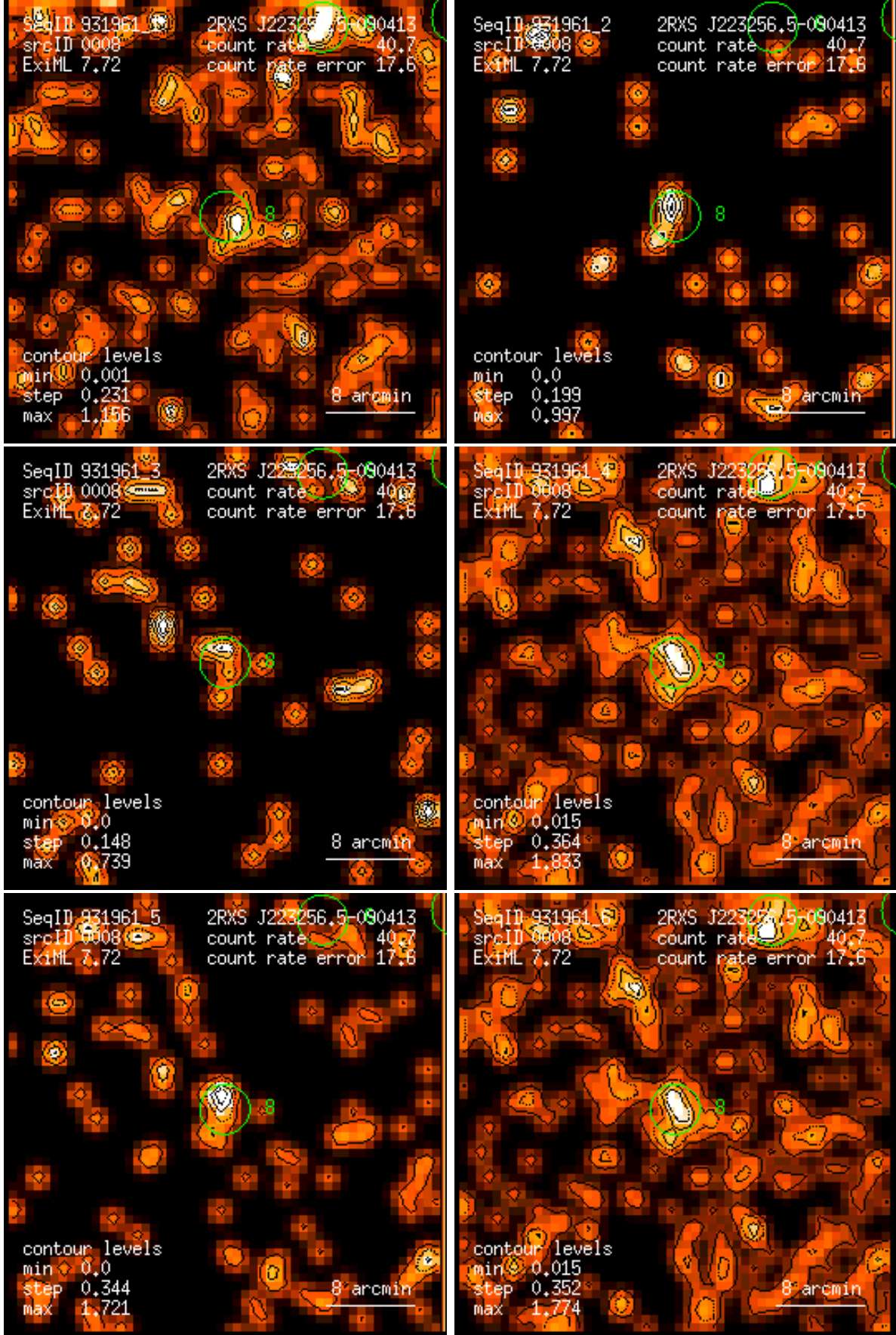
Figure 8: RASS 931961: detection 0008: band rate images, Gaussian filter: (1) PSPC channels 11 – 41, (2) 52 – 90, (3) 91 – 201, (4) 11 – 235, (5) 52 – 201, (6) 11 – 201. Broad band rates in counts/ks. Band rate contour levels in counts/ks/arcmin 2 .
