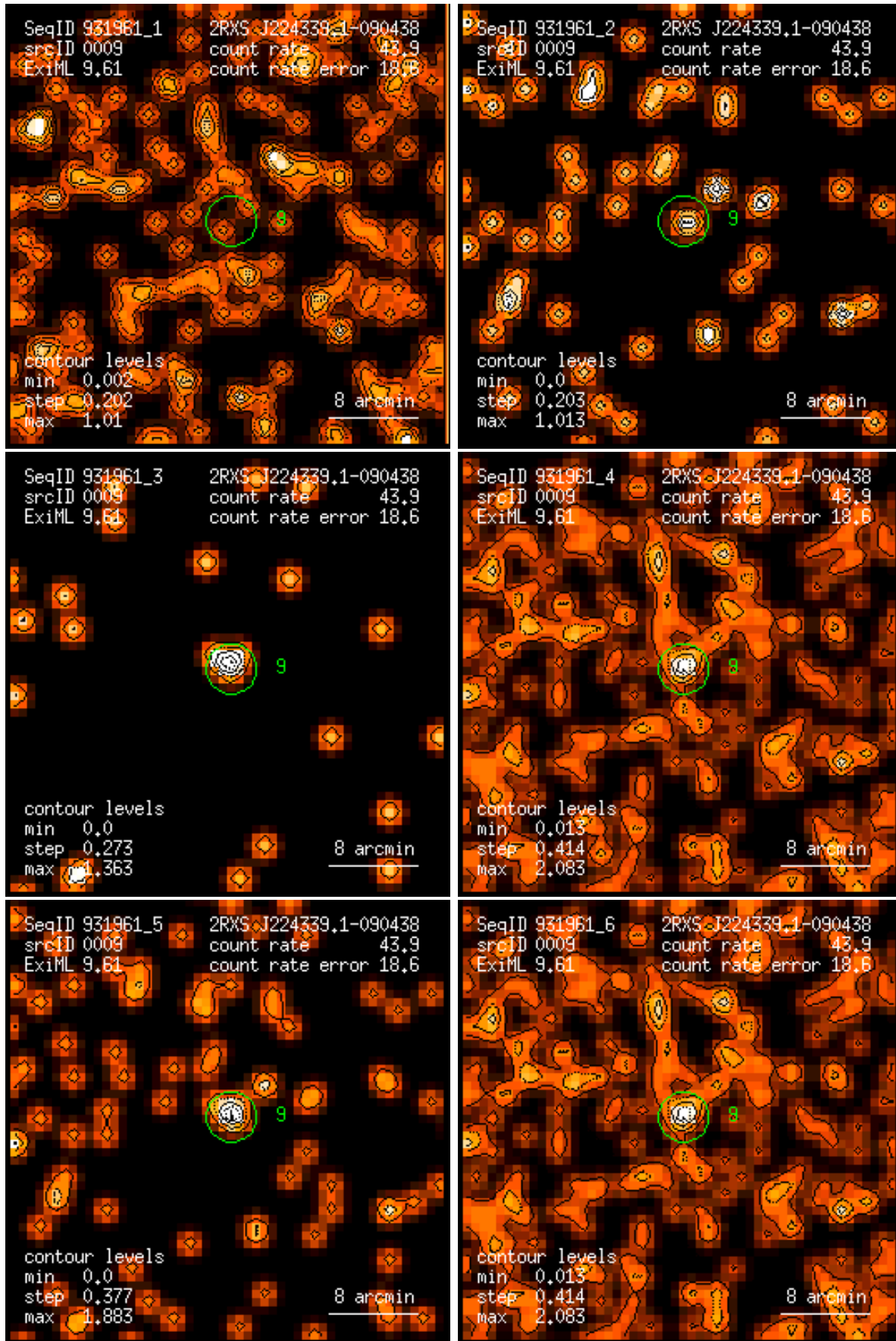
Figure 9: RASS 931961: detection 0009: band rate images, Gaussian filter: (1) PSPC channels 11 – 41, (2) 52 – 90, (3) 91 – 201, (4) 11 – 235, (5) 52 – 201, (6) 11 – 201. Broad band rates in counts/ks. Band rate contour levels in counts/ks/arcmin 2 .
