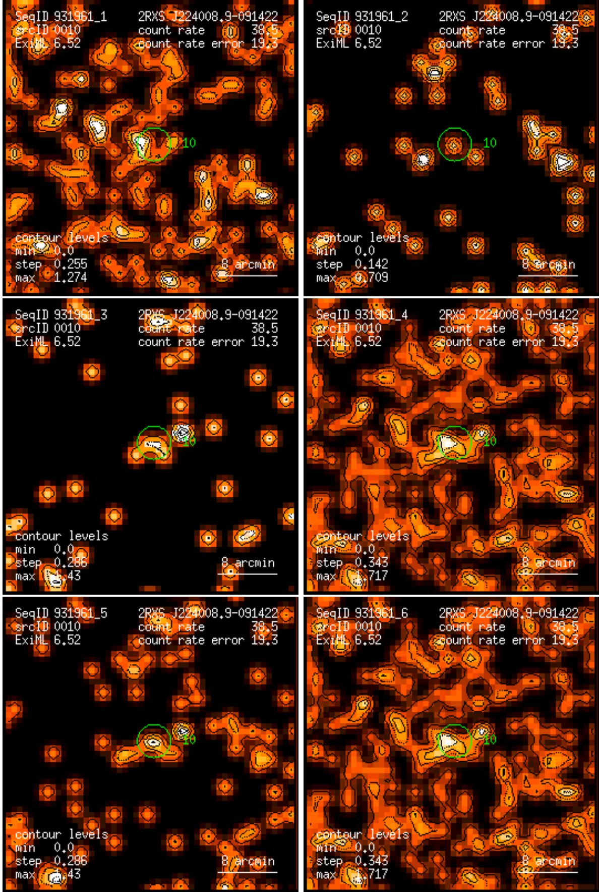
Figure 10: RASS 931961: detection 0010: band rate images, Gaussian filter: (1) PSPC channels 11 – 41, (2) 52 – 90, (3) 91 – 201, (4) 11 – 235, (5) 52 – 201, (6) 11 – 201. Broad band rates in counts/ks. Band rate contour levels in counts/ks/arcmin 2 .
