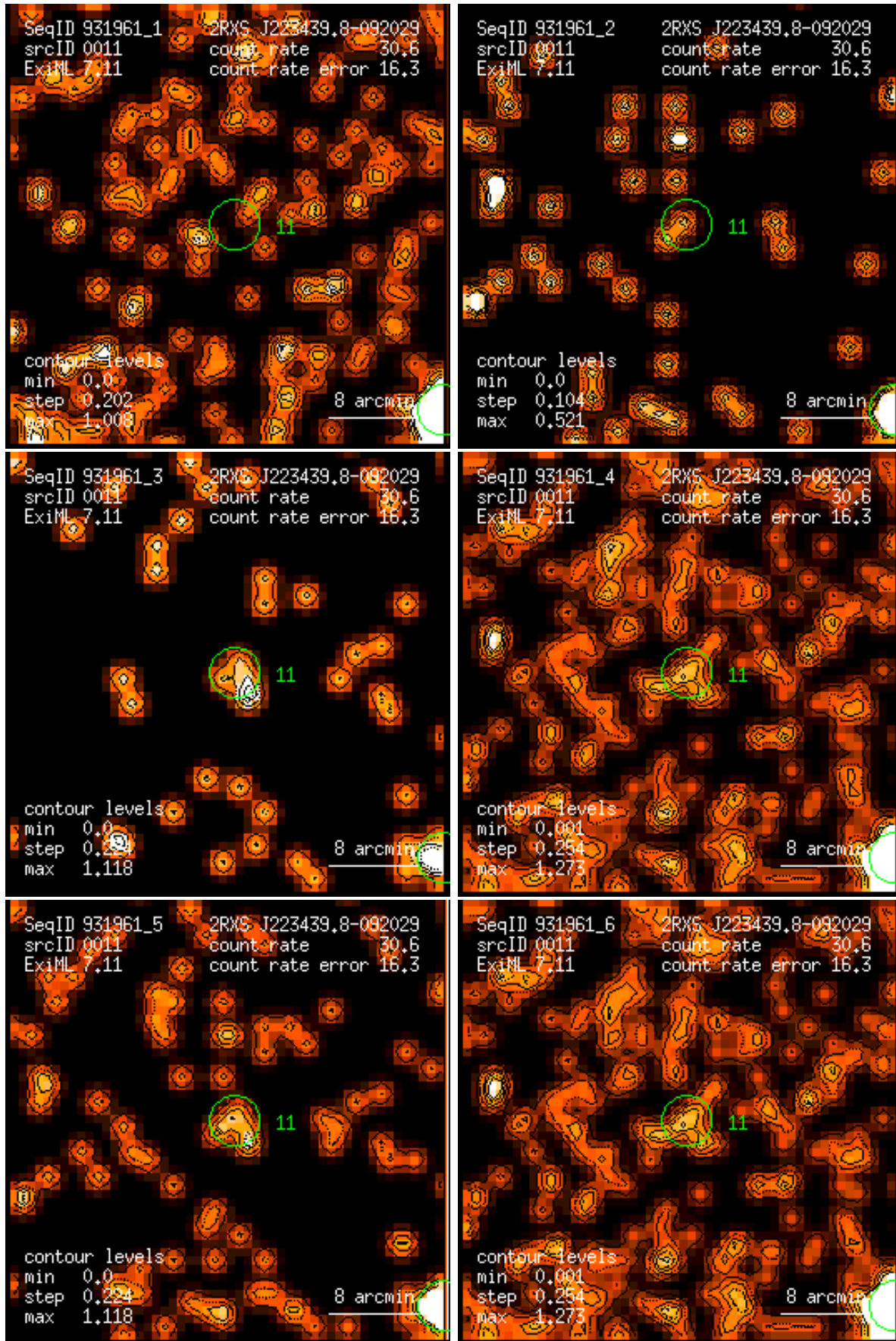
Figure 11: RASS 931961: detection 0011: band rate images, Gaussian filter: (1) PSPC channels 11 – 41, (2) 52 – 90, (3) 91 – 201, (4) 11 – 235, (5) 52 – 201, (6) 11 – 201. Broad band rates in counts/ks. Band rate contour levels in counts/ks/arcmin 2 .
