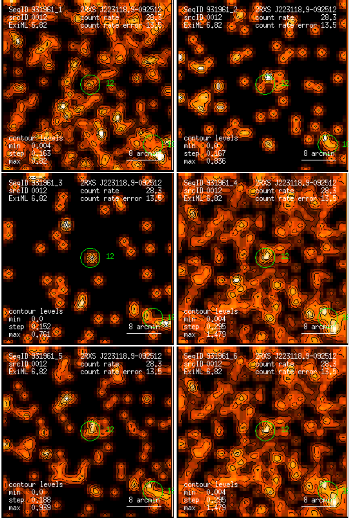
Figure 12: RASS 931961: detection 0012: band rate images, Gaussian filter: (1) PSPC channels 11 – 41, (2) 52 – 90, (3) 91 – 201, (4) 11 – 235, (5) 52 – 201, (6) 11 – 201. Broad band rates in counts/ks. Band rate contour levels in counts/ks/arcmin 2 .
