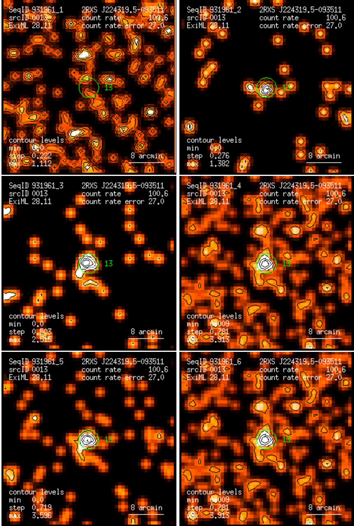
Figure 13: RASS 931961: detection 0013: band rate images, Gaussian filter: (1) PSPC channels 11 – 41, (2) 52 – 90, (3) 91 – 201, (4) 11 – 235, (5) 52 – 201, (6) 11 – 201. Broad band rates in counts/ks. Band rate contour levels in counts/ks/arcmin 2 .
