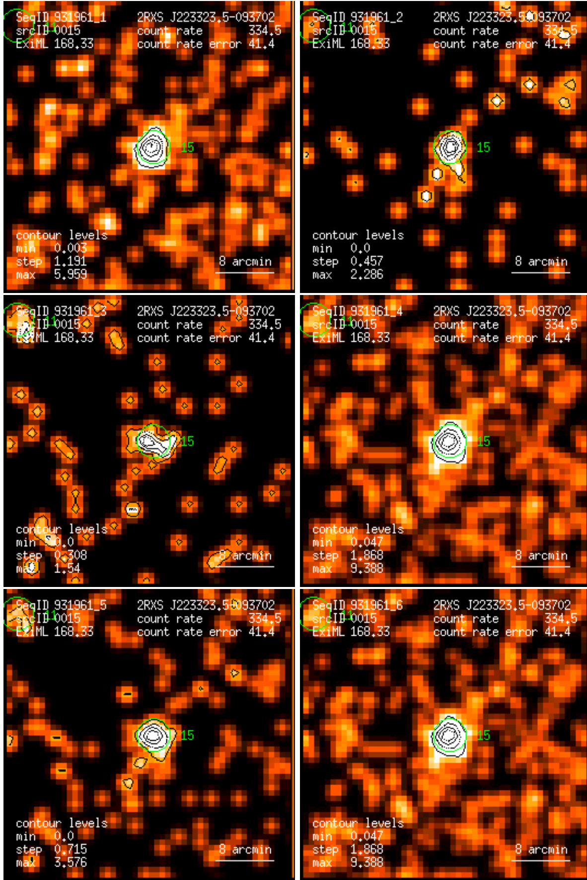
Figure 15: RASS 931961: detection 0015: band rate images, Gaussian filter: (1) PSPC channels 11 – 41, (2) 52 – 90, (3) 91 – 201, (4) 11 – 235, (5) 52 – 201, (6) 11 – 201. Broad band rates in counts/ks. Band rate contour levels in counts/ks/arcmin 2 .
