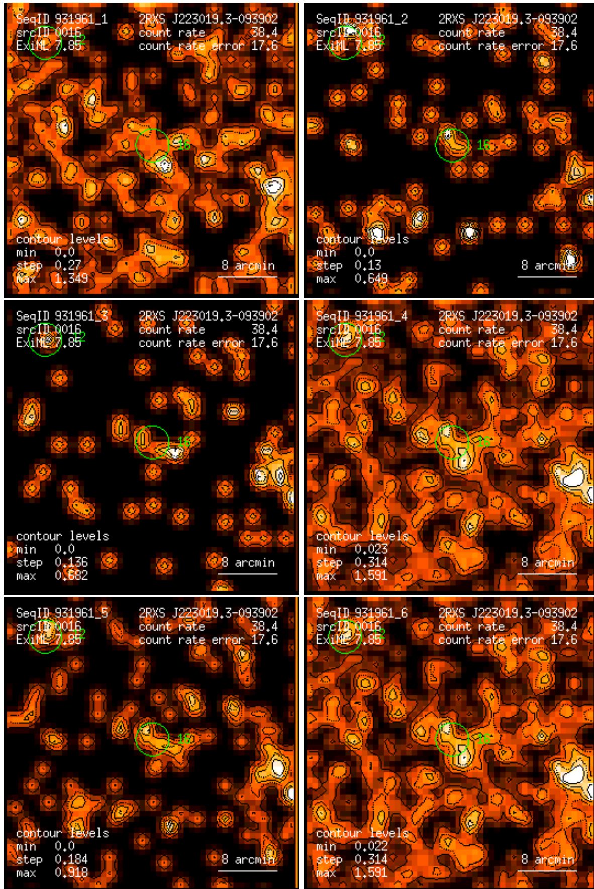
Figure 16: RASS 931961: detection 0016: band rate images, Gaussian filter: (1) PSPC channels 11 – 41, (2) 52 – 90, (3) 91 – 201, (4) 11 – 235, (5) 52 – 201, (6) 11 – 201. Broad band rates in counts/ks. Band rate contour levels in counts/ks/arcmin 2 .
