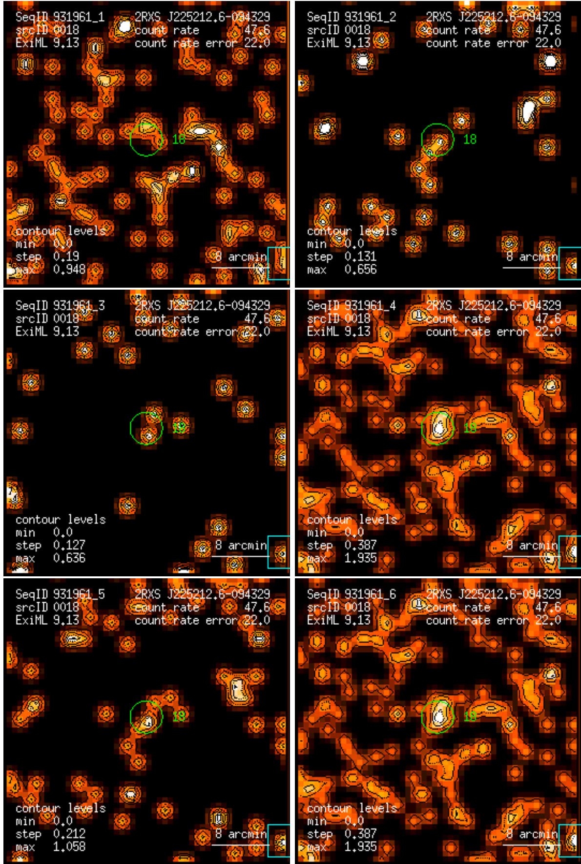
Figure 18: RASS 931961: detection 0018: band rate images, Gaussian filter: (1) PSPC channels 11 – 41, (2) 52 – 90, (3) 91 – 201, (4) 11 – 235, (5) 52 – 201, (6) 11 – 201. Broad band rates in counts/ks. Band rate contour levels in counts/ks/arcmin 2 .
