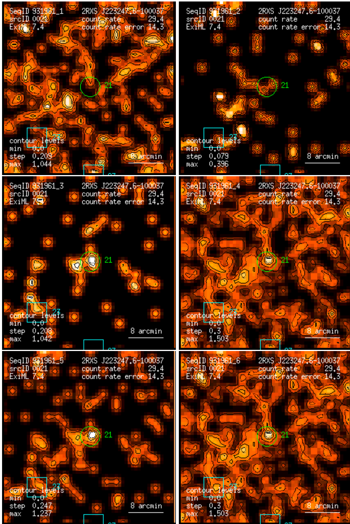
Figure 21: RASS 931961: detection 0021: band rate images, Gaussian filter: (1) PSPC channels 11 – 41, (2) 52 – 90, (3) 91 – 201, (4) 11 – 235, (5) 52 – 201, (6) 11 – 201. Broad band rates in counts/ks. Band rate contour levels in counts/ks/arcmin 2 .
