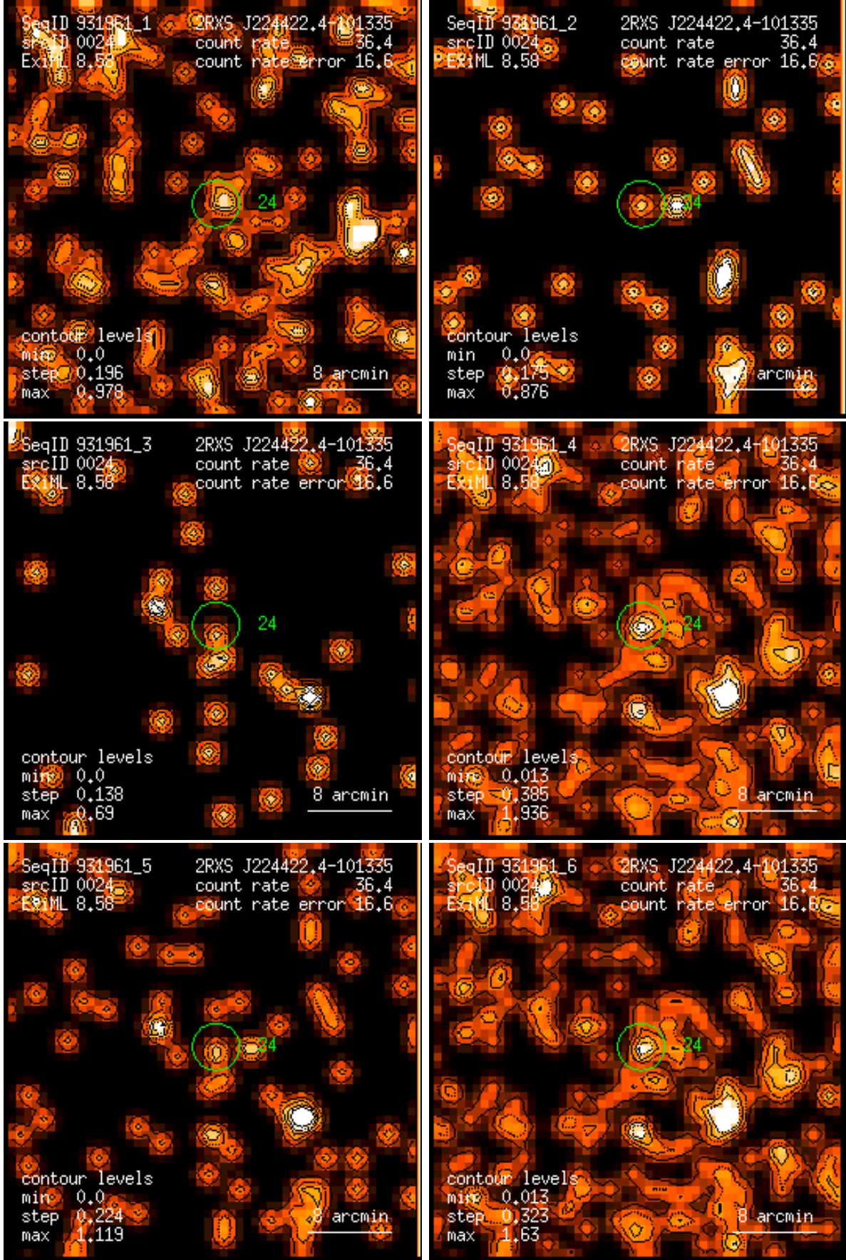
Figure 24: RASS 931961: detection 0024: band rate images, Gaussian filter: (1) PSPC channels 11 – 41, (2) 52 – 90, (3) 91 – 201, (4) 11 – 235, (5) 52 – 201, (6) 11 – 201. Broad band rates in counts/ks. Band rate contour levels in counts/ks/arcmin 2 .
