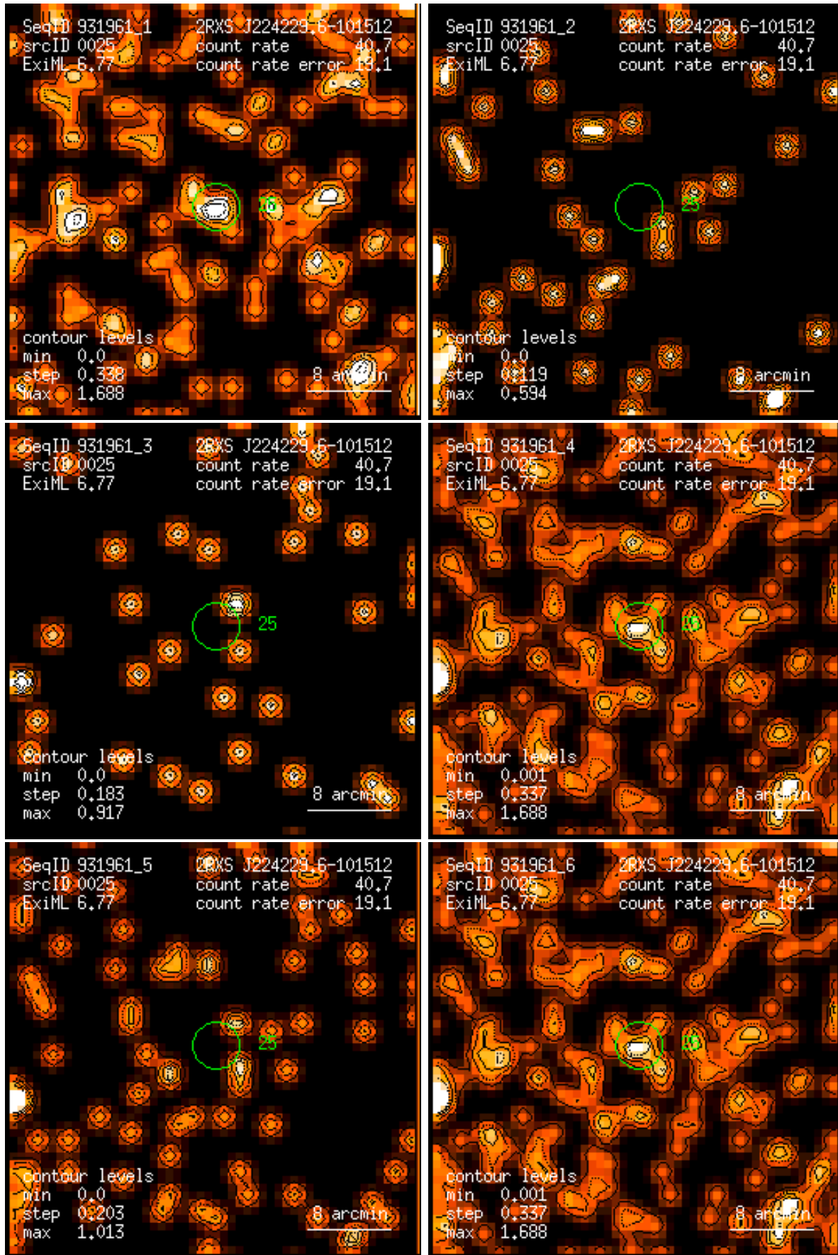
Figure 25: RASS 931961: detection 0025: band rate images, Gaussian filter: (1) PSPC channels 11 – 41, (2) 52 – 90, (3) 91 – 201, (4) 11 – 235, (5) 52 – 201, (6) 11 – 201. Broad band rates in counts/ks. Band rate contour levels in counts/ks/arcmin 2 .
