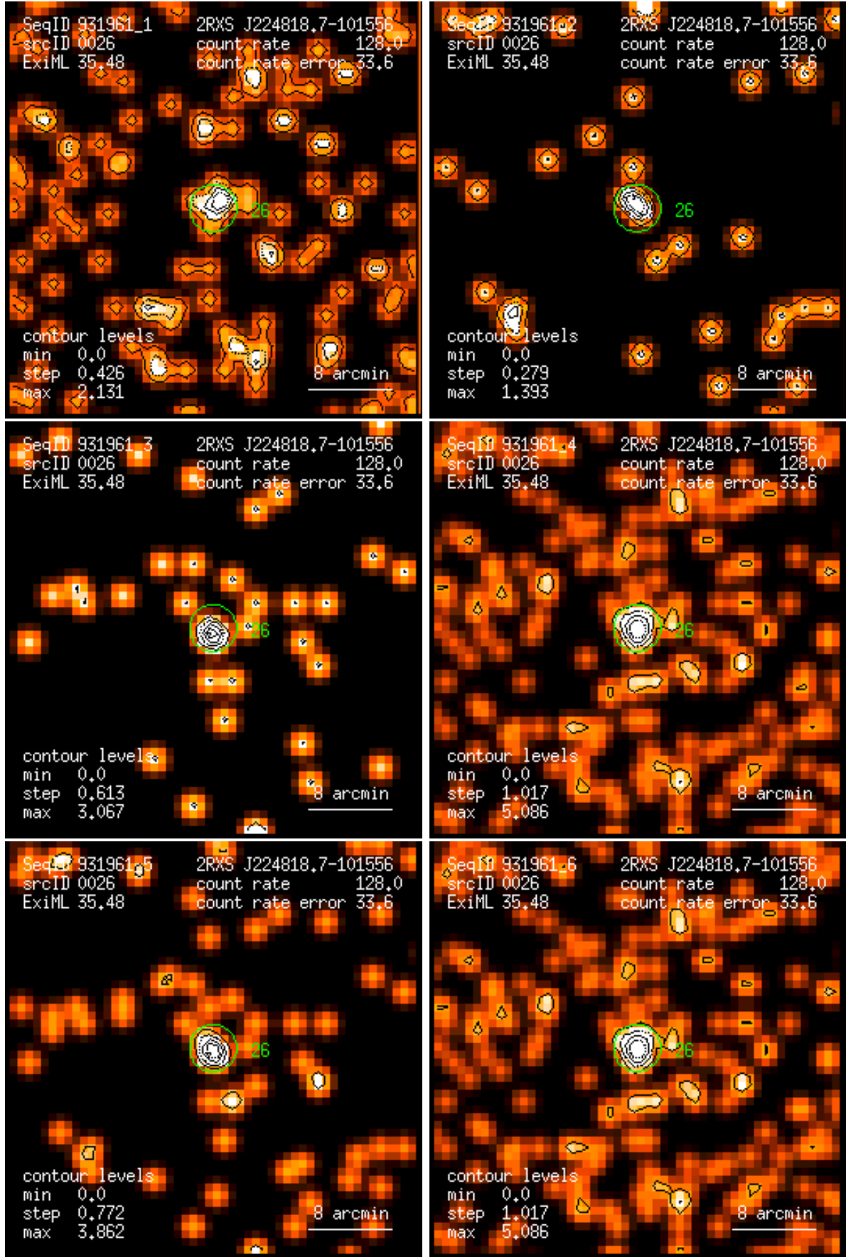
Figure 26: RASS 931961: detection 0026: band rate images, Gaussian filter: (1) PSPC channels 11 – 41, (2) 52 – 90, (3) 91 – 201, (4) 11 – 235, (5) 52 – 201, (6) 11 – 201. Broad band rates in counts/ks. Band rate contour levels in counts/ks/arcmin 2 .
