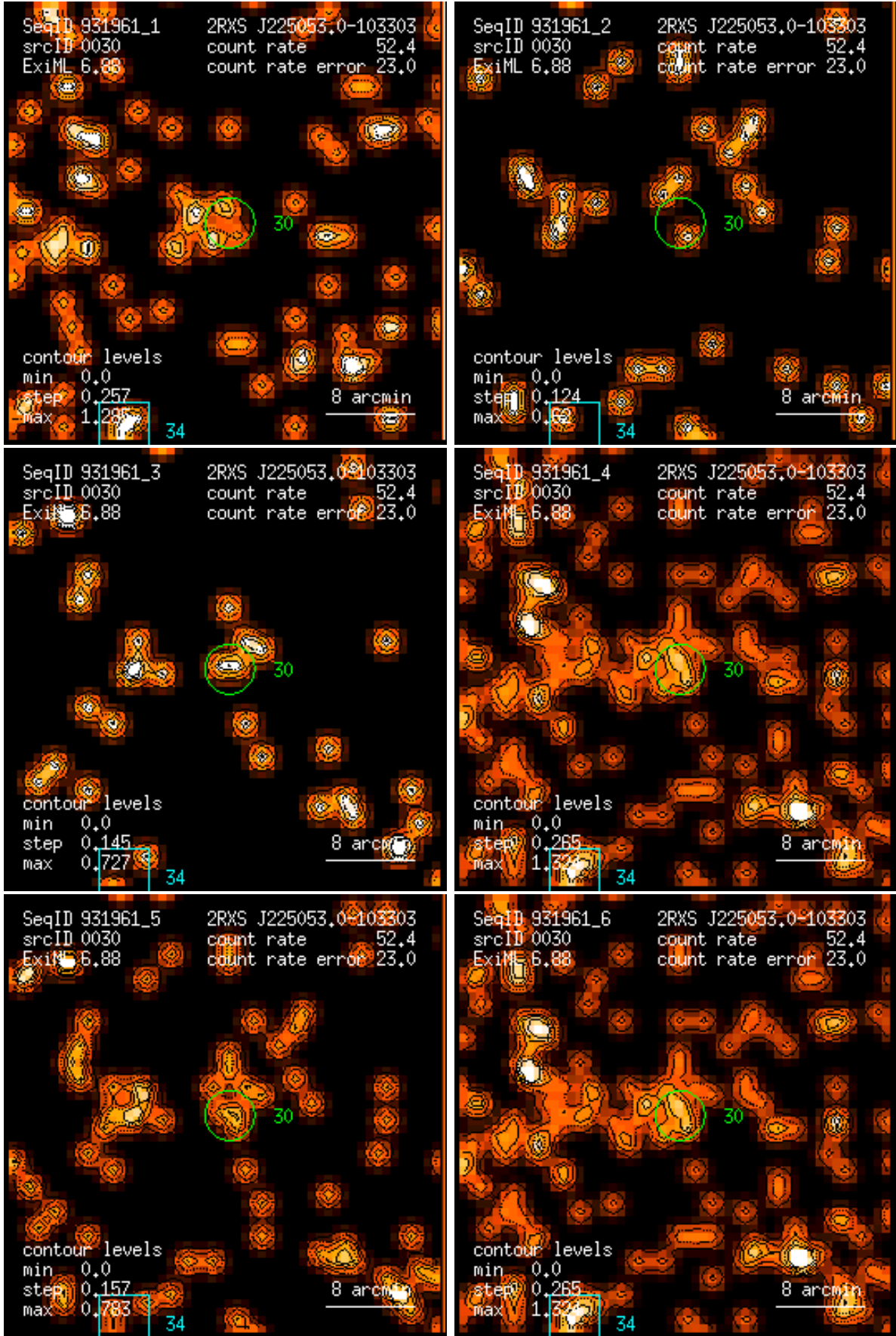
Figure 30: RASS 931961: detection 0030: band rate images, Gaussian filter: (1) PSPC channels 11 – 41, (2) 52 – 90, (3) 91 – 201, (4) 11 – 235, (5) 52 – 201, (6) 11 – 201. Broad band rates in counts/ks. Band rate contour levels in counts/ks/arcmin 2 .
