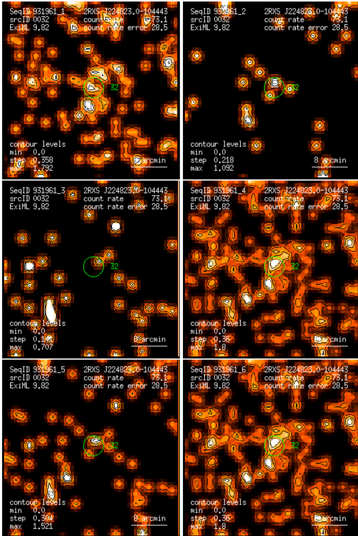
Figure 32: RASS 931961: detection 0032: band rate images, Gaussian filter: (1) PSPC channels 11 – 41, (2) 52 – 90, (3) 91 – 201, (4) 11 – 235, (5) 52 – 201, (6) 11 – 201. Broad band rates in counts/ks. Band rate contour levels in counts/ks/arcmin 2 .
