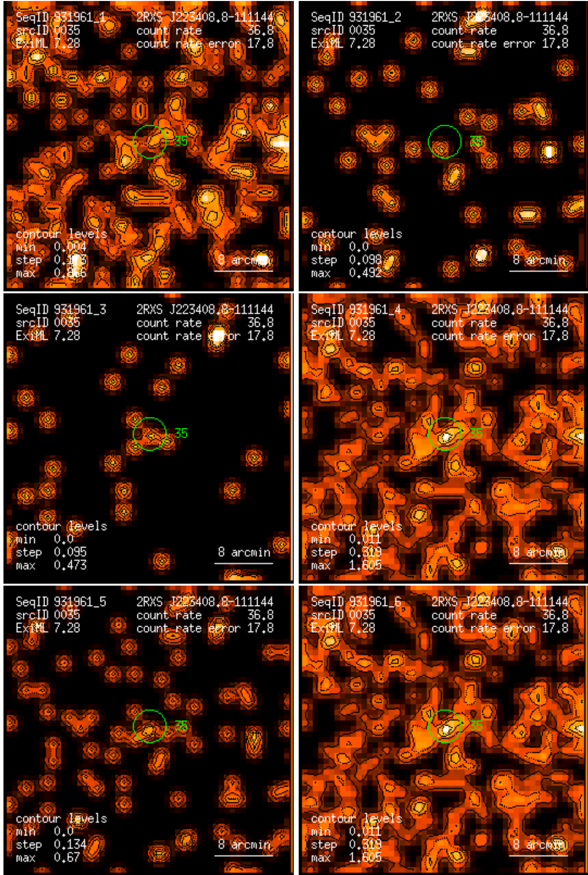
Figure 35: RASS 931961: detection 0035: band rate images, Gaussian filter: (1) PSPC channels 11 – 41, (2) 52 – 90, (3) 91 – 201, (4) 11 – 235, (5) 52 – 201, (6) 11 – 201. Broad band rates in counts/ks. Band rate contour levels in counts/ks/arcmin 2 .
