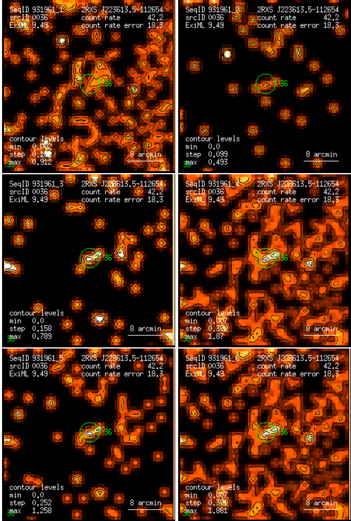
Figure 36: RASS 931961: detection 0036: band rate images, Gaussian filter: (1) PSPC channels 11 – 41, (2) 52 – 90, (3) 91 – 201, (4) 11 – 235, (5) 52 – 201, (6) 11 – 201. Broad band rates in counts/ks. Band rate contour levels in counts/ks/arcmin 2 .
