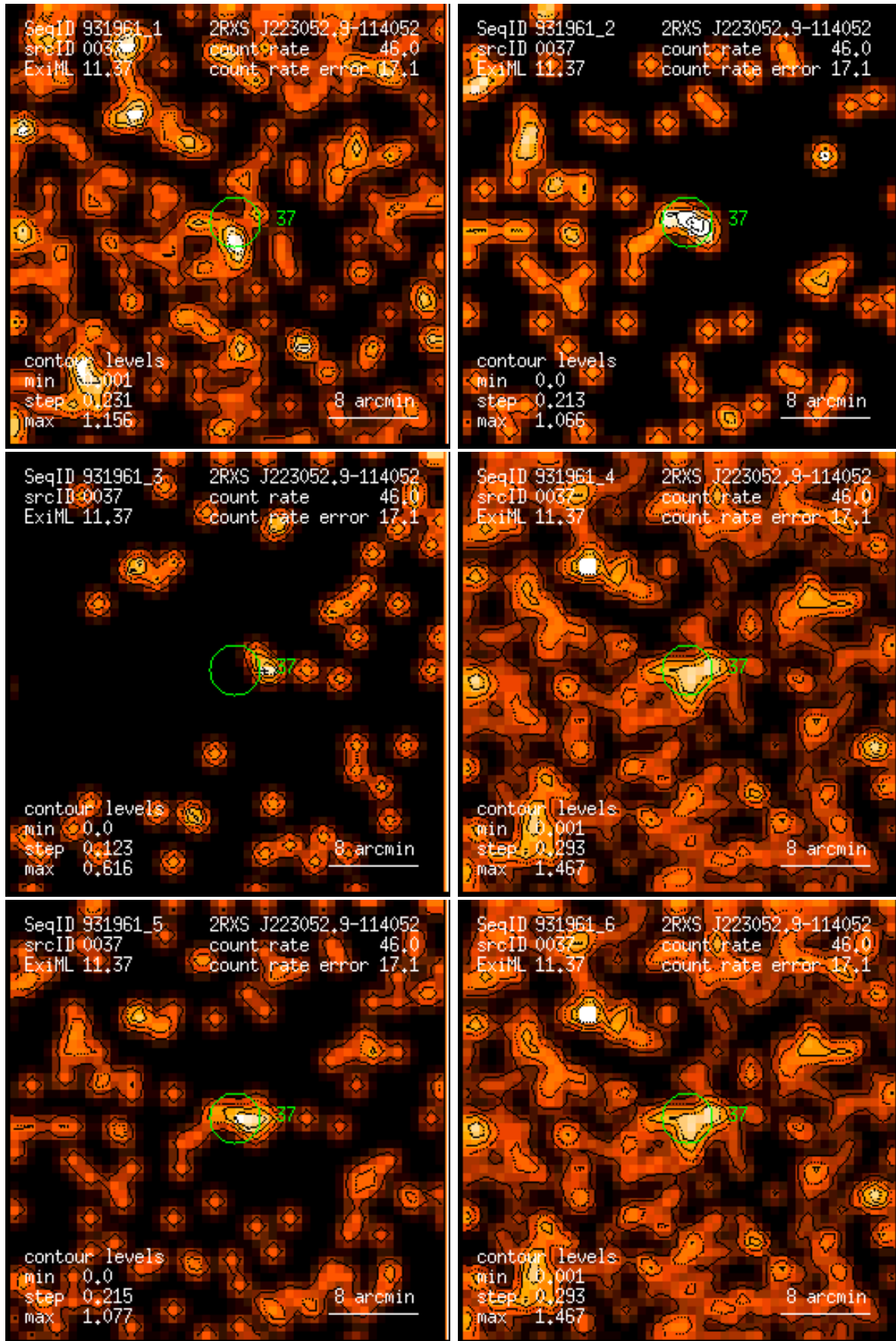
Figure 37: RASS 931961: detection 0037: band rate images, Gaussian filter: (1) PSPC channels 11 – 41, (2) 52 – 90, (3) 91 – 201, (4) 11 – 235, (5) 52 – 201, (6) 11 – 201. Broad band rates in counts/ks. Band rate contour levels in counts/ks/arcmin 2 .
