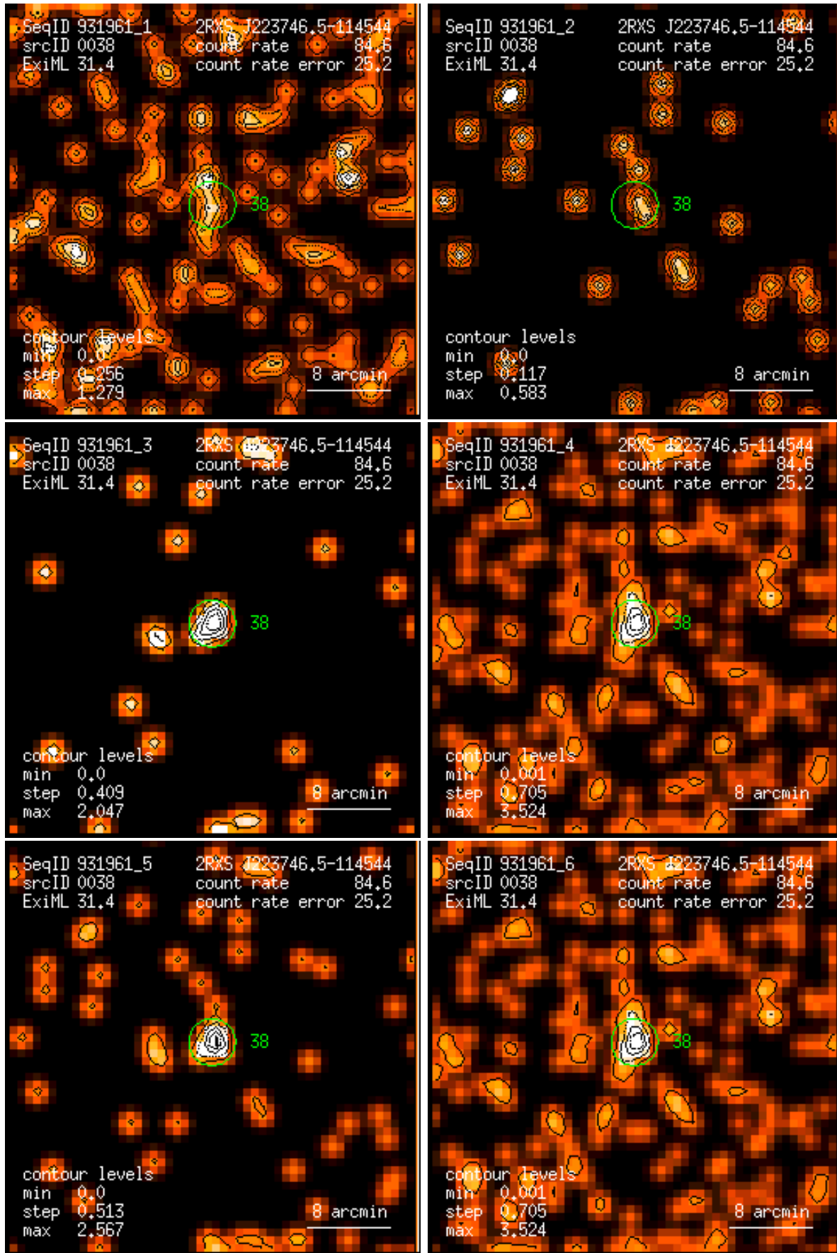
Figure 38: RASS 931961: detection 0038: band rate images, Gaussian filter: (1) PSPC channels 11 – 41, (2) 52 – 90, (3) 91 – 201, (4) 11 – 235, (5) 52 – 201, (6) 11 – 201. Broad band rates in counts/ks. Band rate contour levels in counts/ks/arcmin 2 .
