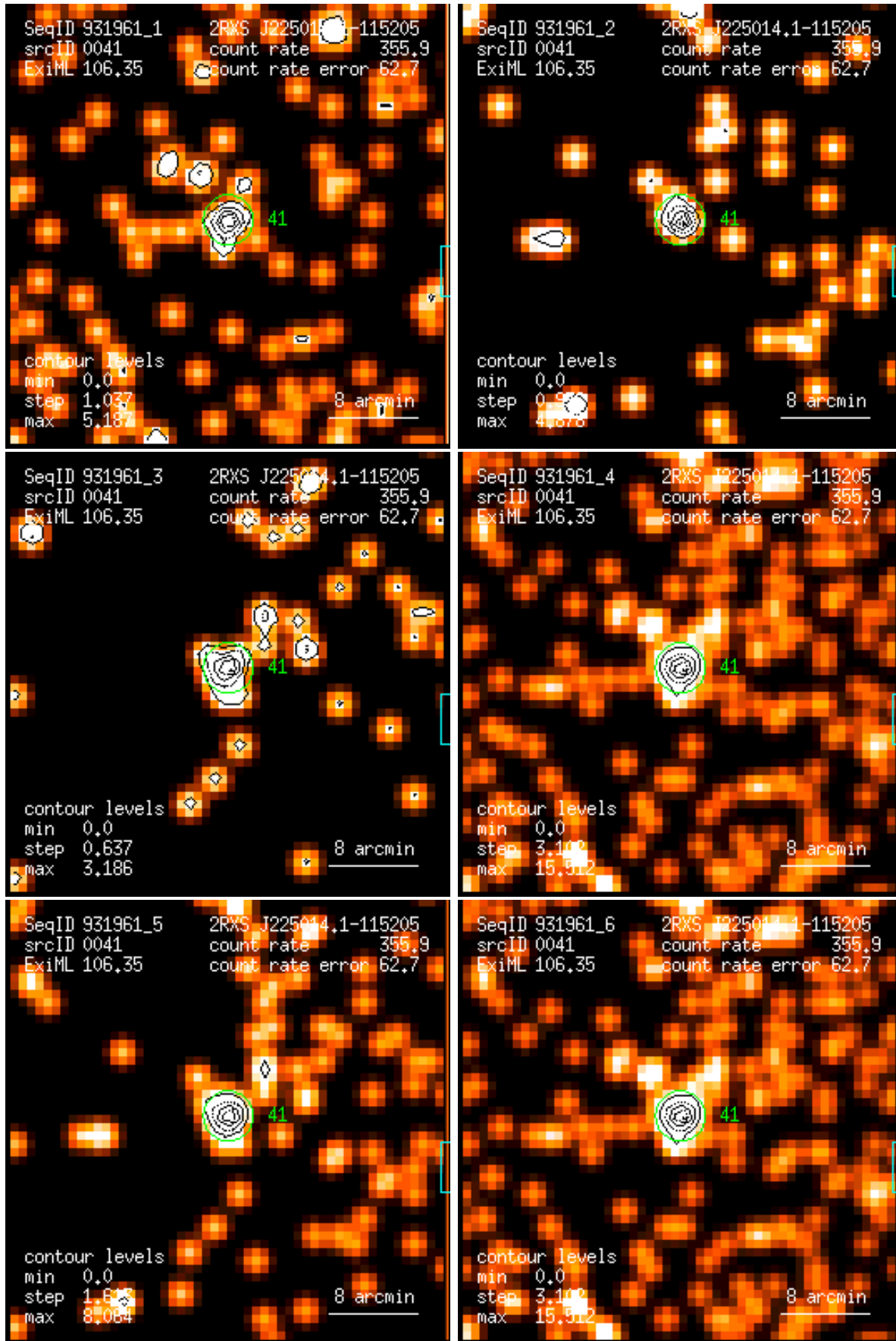
Figure 41: RASS 931961: detection 0041: band rate images, Gaussian filter: (1) PSPC channels 11 – 41, (2) 52 – 90, (3) 91 – 201, (4) 11 – 235, (5) 52 – 201, (6) 11 – 201. Broad band rates in counts/ks. Band rate contour levels in counts/ks/arcmin 2 .
