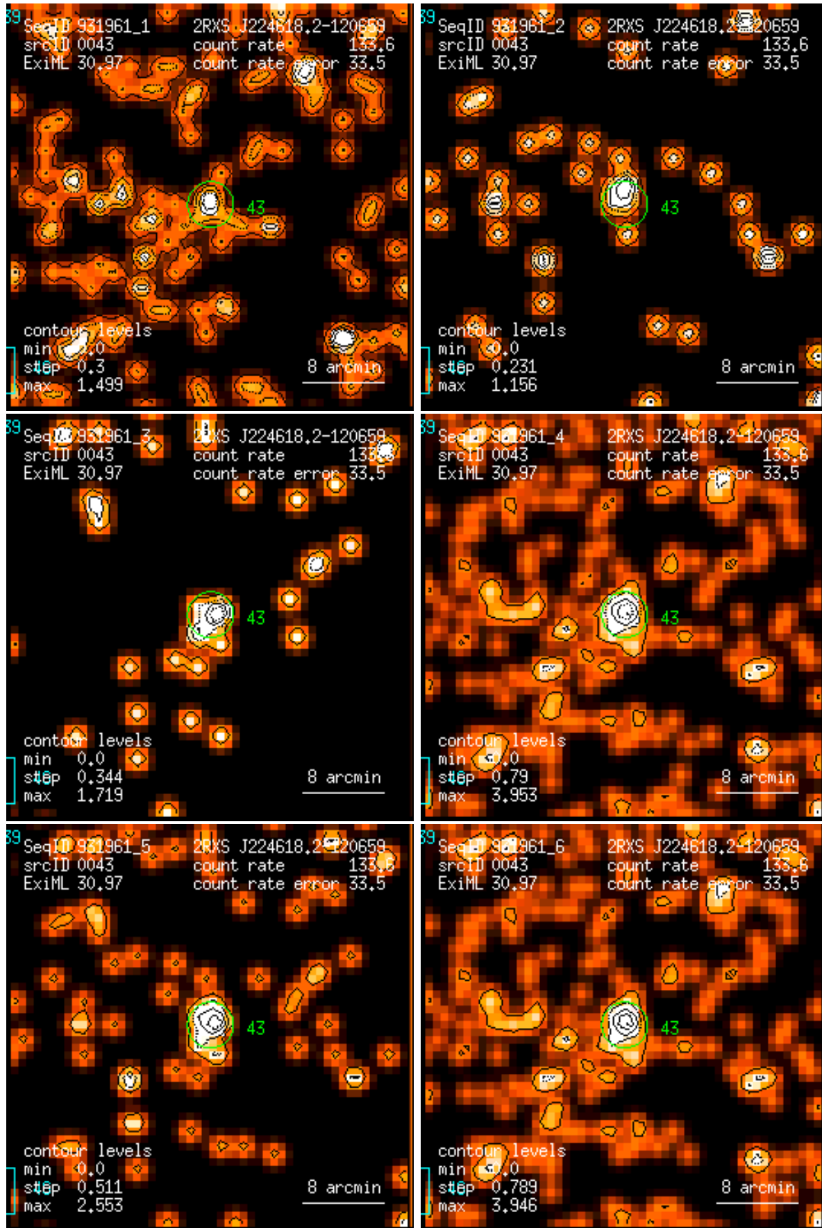
Figure 43: RASS 931961: detection 0043: band rate images, Gaussian filter: (1) PSPC channels 11 – 41, (2) 52 – 90, (3) 91 – 201, (4) 11 – 235, (5) 52 – 201, (6) 11 – 201. Broad band rates in counts/ks. Band rate contour levels in counts/ks/arcmin 2 .
