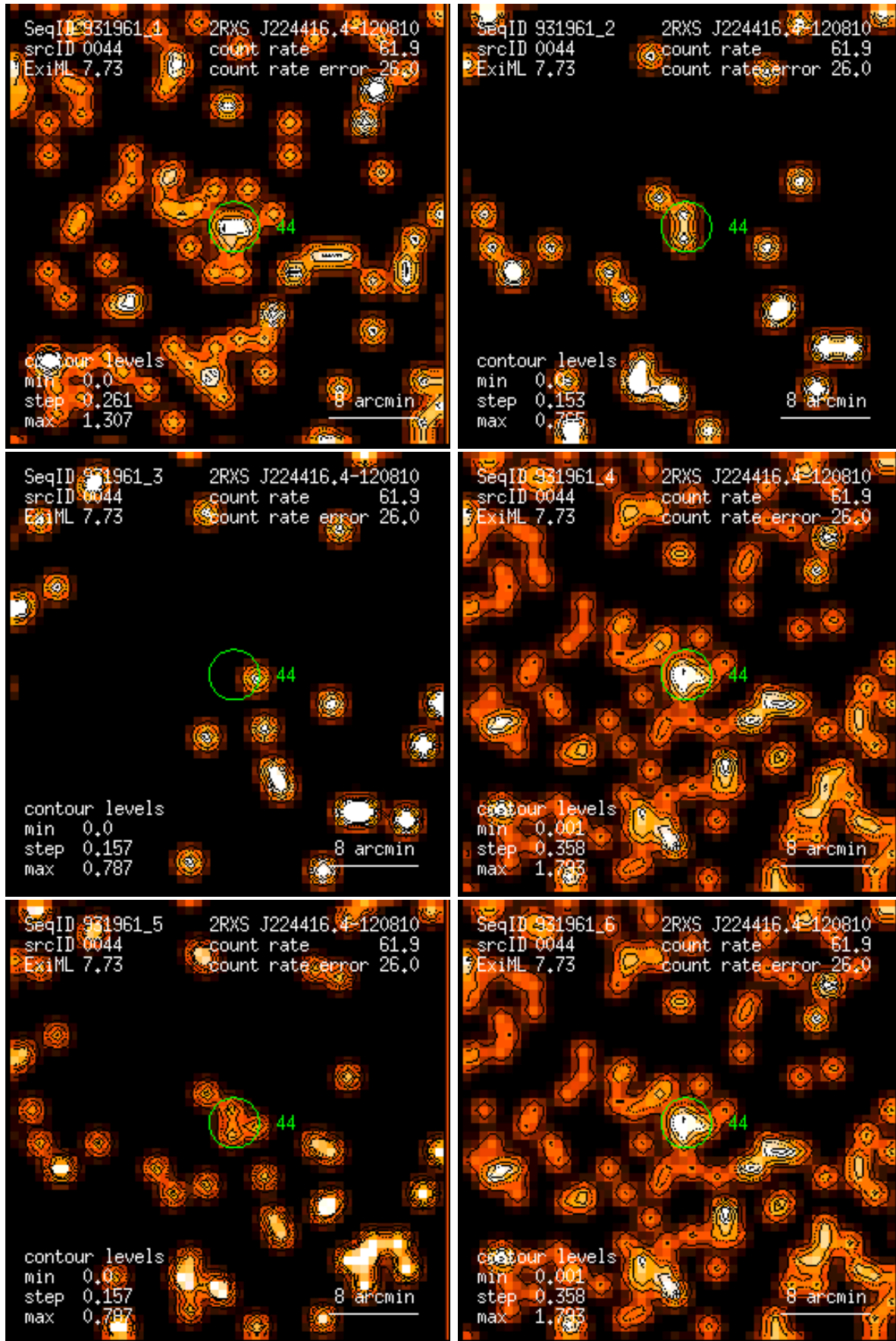
Figure 44: RASS 931961: detection 0044: band rate images, Gaussian filter: (1) PSPC channels 11 – 41, (2) 52 – 90, (3) 91 – 201, (4) 11 – 235, (5) 52 – 201, (6) 11 – 201. Broad band rates in counts/ks. Band rate contour levels in counts/ks/arcmin 2 .
