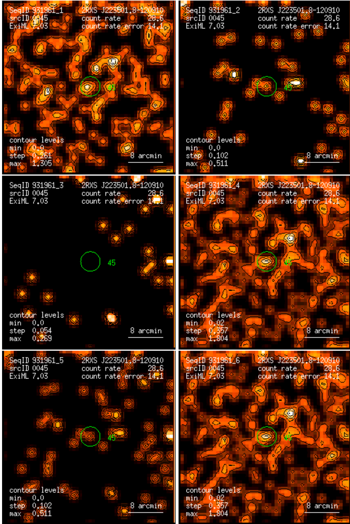
Figure 45: RASS 931961: detection 0045: band rate images, Gaussian filter: (1) PSPC channels 11 – 41, (2) 52 – 90, (3) 91 – 201, (4) 11 – 235, (5) 52 – 201, (6) 11 – 201. Broad band rates in counts/ks. Band rate contour levels in counts/ks/arcmin 2 .
