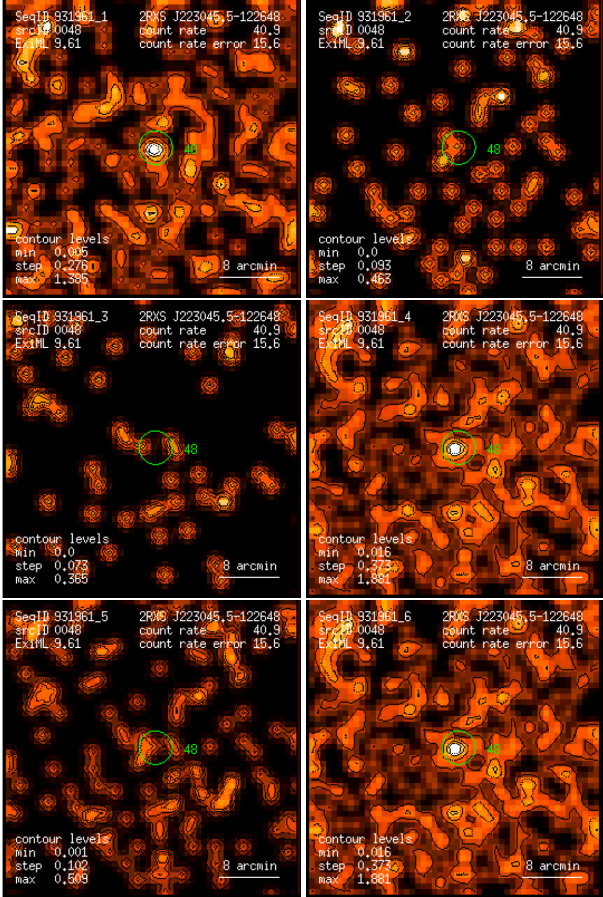
Figure 48: RASS 931961: detection 0048: band rate images, Gaussian filter: (1) PSPC channels 11 – 41, (2) 52 – 90, (3) 91 – 201, (4) 11 – 235, (5) 52 – 201, (6) 11 – 201. Broad band rates in counts/ks. Band rate contour levels in counts/ks/arcmin 2 .
