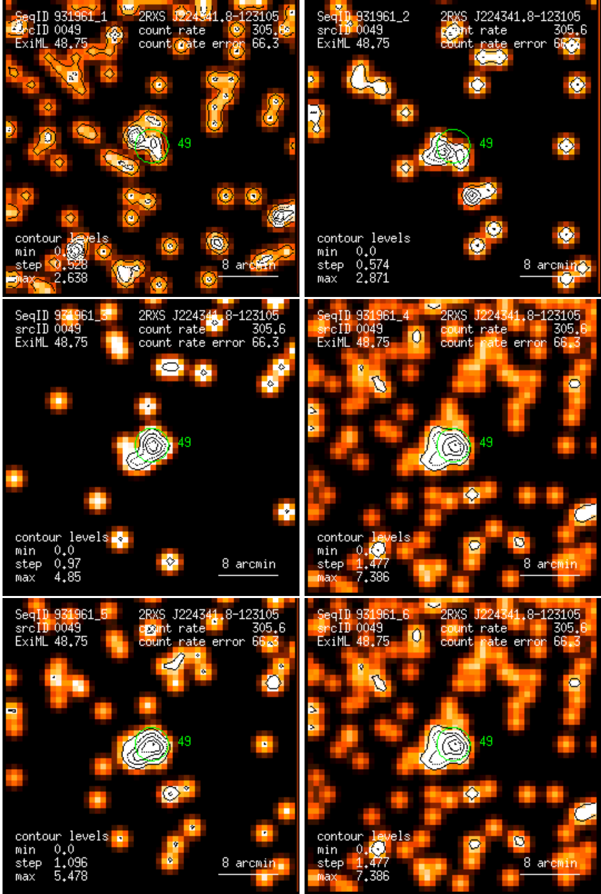
Figure 49: RASS 931961: detection 0049: band rate images, Gaussian filter: (1) PSPC channels 11 – 41, (2) 52 – 90, (3) 91 – 201, (4) 11 – 235, (5) 52 – 201, (6) 11 – 201. Broad band rates in counts/ks. Band rate contour levels in counts/ks/arcmin 2 .
