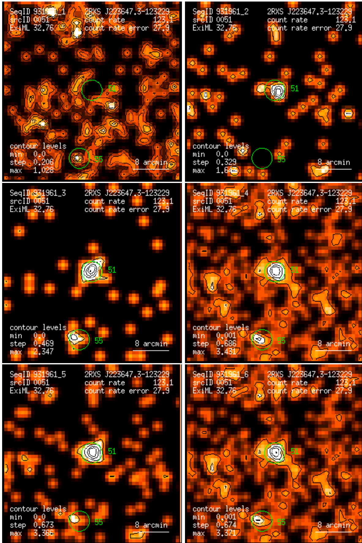
Figure 51: RASS 931961: detection 0051: band rate images, Gaussian filter: (1) PSPC channels 11 – 41, (2) 52 – 90, (3) 91 – 201, (4) 11 – 235, (5) 52 – 201, (6) 11 – 201. Broad band rates in counts/ks. Band rate contour levels in counts/ks/arcmin 2 .
