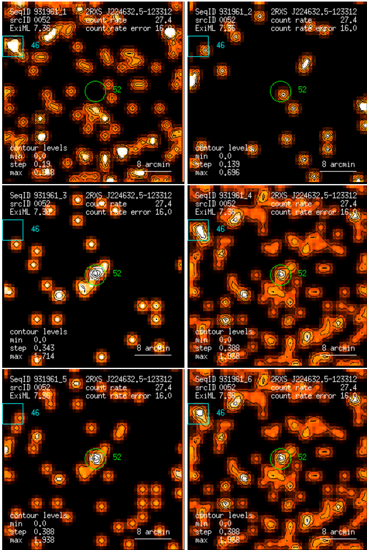
Figure 52: RASS 931961: detection 0052: band rate images, Gaussian filter: (1) PSPC channels 11 – 41, (2) 52 – 90, (3) 91 – 201, (4) 11 – 235, (5) 52 – 201, (6) 11 – 201. Broad band rates in counts/ks. Band rate contour levels in counts/ks/arcmin 2 .
