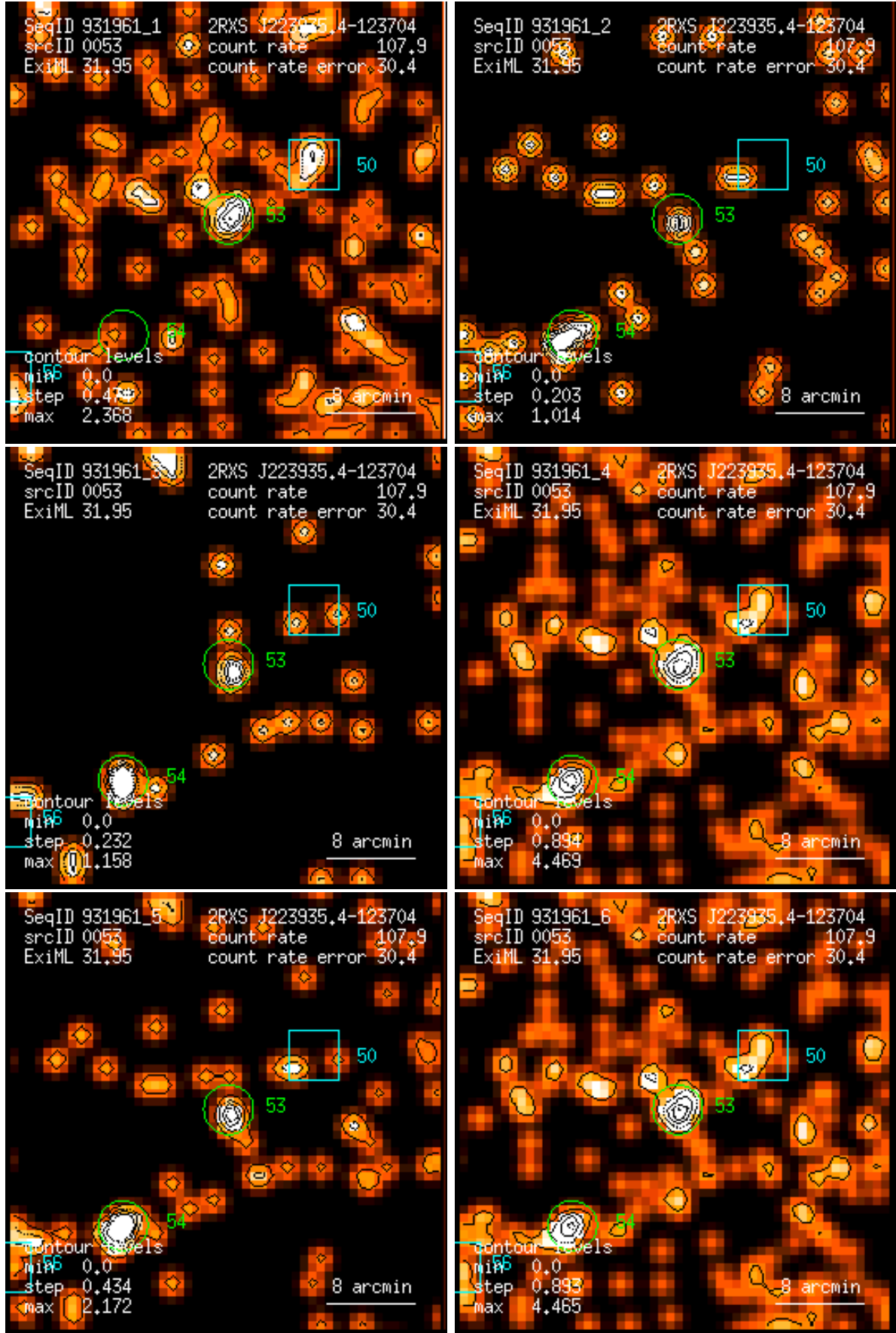
Figure 53: RASS 931961: detection 0053: band rate images, Gaussian filter: (1) PSPC channels 11 – 41, (2) 52 – 90, (3) 91 – 201, (4) 11 – 235, (5) 52 – 201, (6) 11 – 201. Broad band rates in counts/ks. Band rate contour levels in counts/ks/arcmin 2 .
