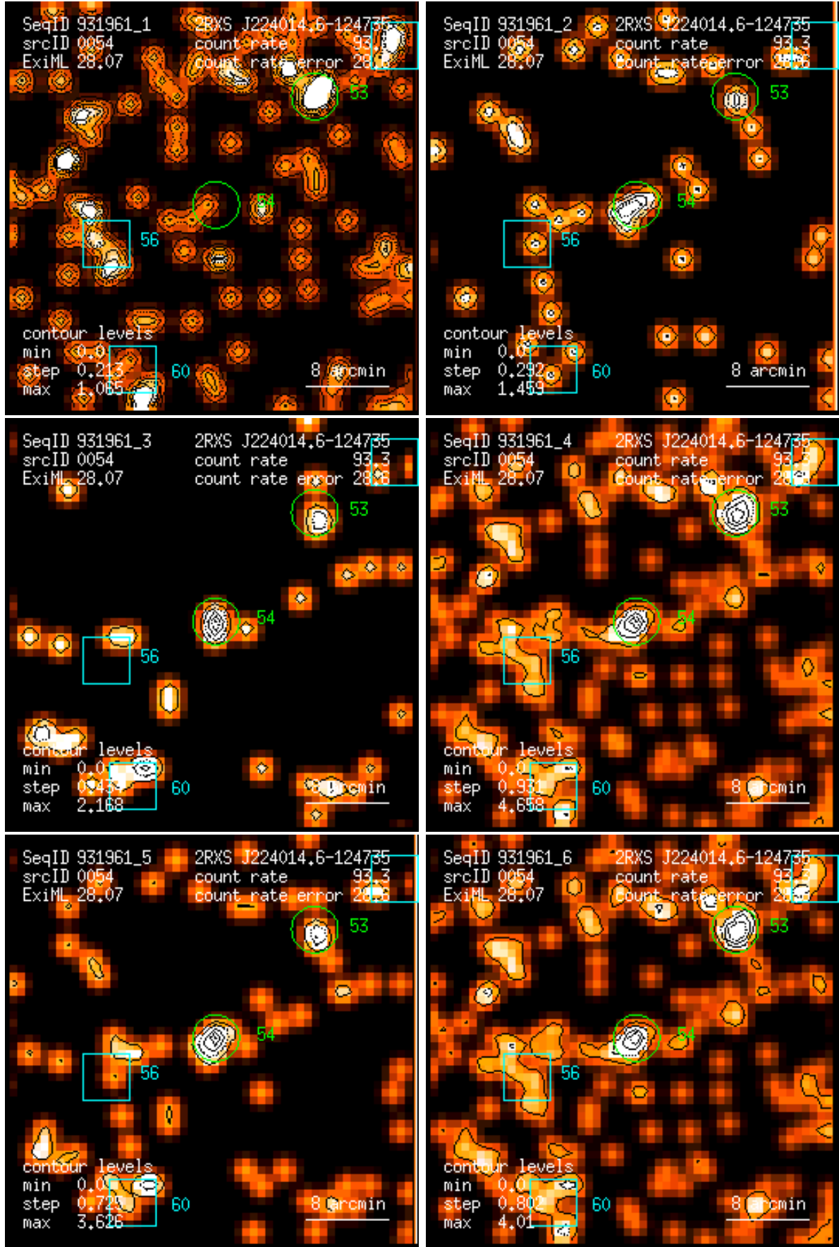
Figure 54: RASS 931961: detection 0054: band rate images, Gaussian filter: (1) PSPC channels 11 – 41, (2) 52 – 90, (3) 91 – 201, (4) 11 – 235, (5) 52 – 201, (6) 11 – 201. Broad band rates in counts/ks. Band rate contour levels in counts/ks/arcmin 2 .
