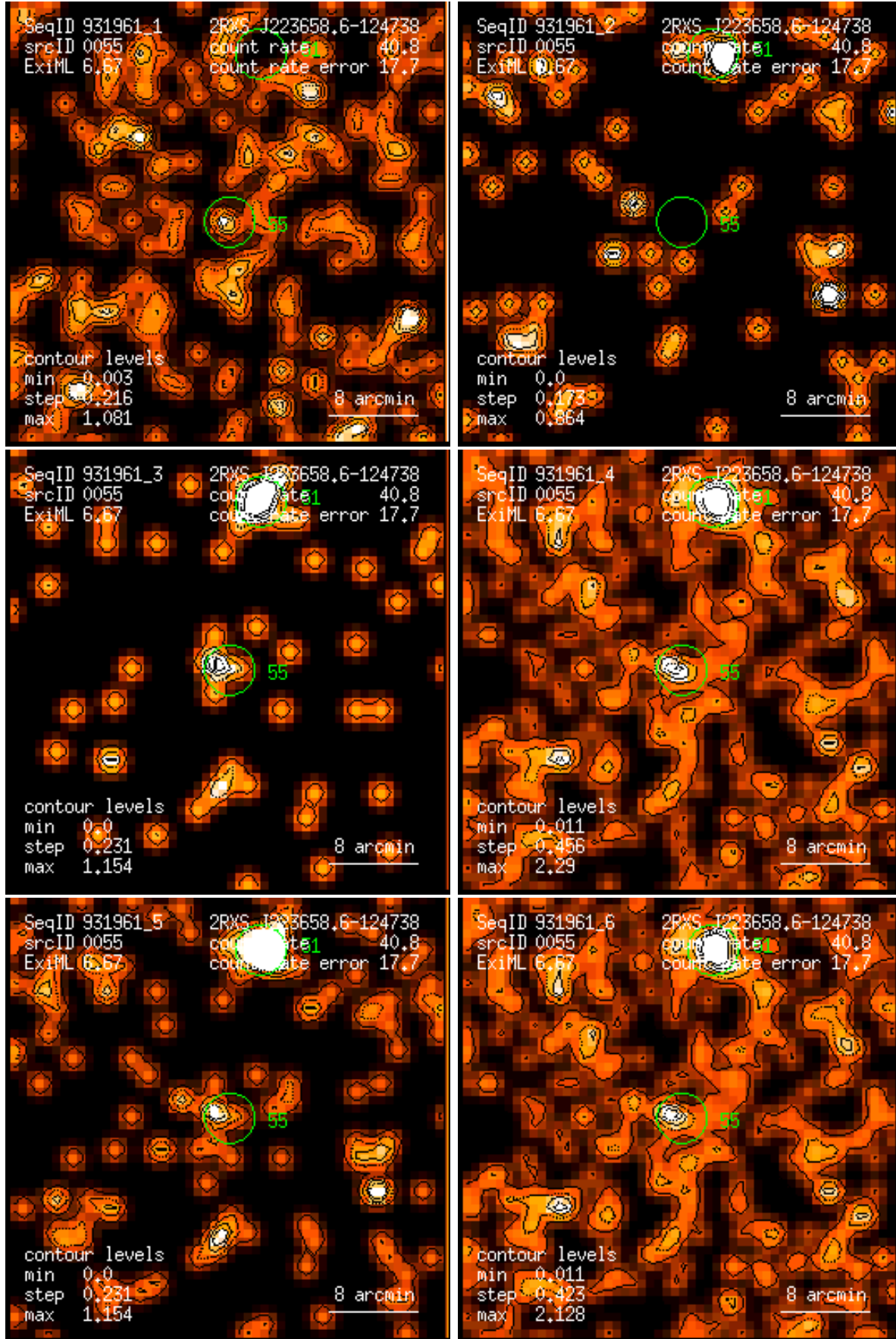
Figure 55: RASS 931961: detection 0055: band rate images, Gaussian filter: (1) PSPC channels 11 – 41, (2) 52 – 90, (3) 91 – 201, (4) 11 – 235, (5) 52 – 201, (6) 11 – 201. Broad band rates in counts/ks. Band rate contour levels in counts/ks/arcmin 2 .
